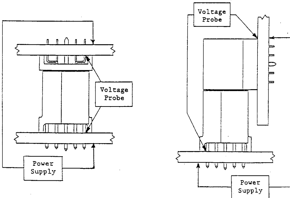
Figure 4 Resistance & Temperature Measurement Points
