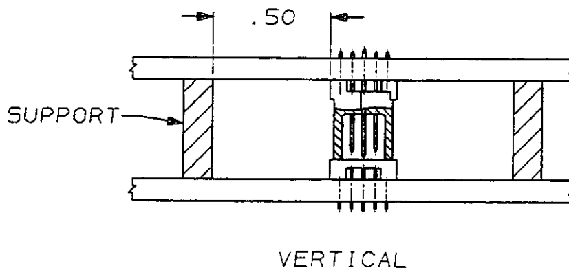
Figure 5 Mounting & Clamping Location For Vibration & Physical Shock
