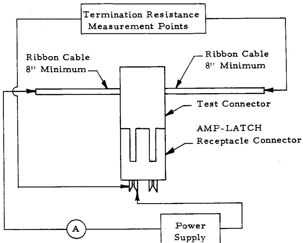
Figure 4 Termination Resistance Measurement Points
