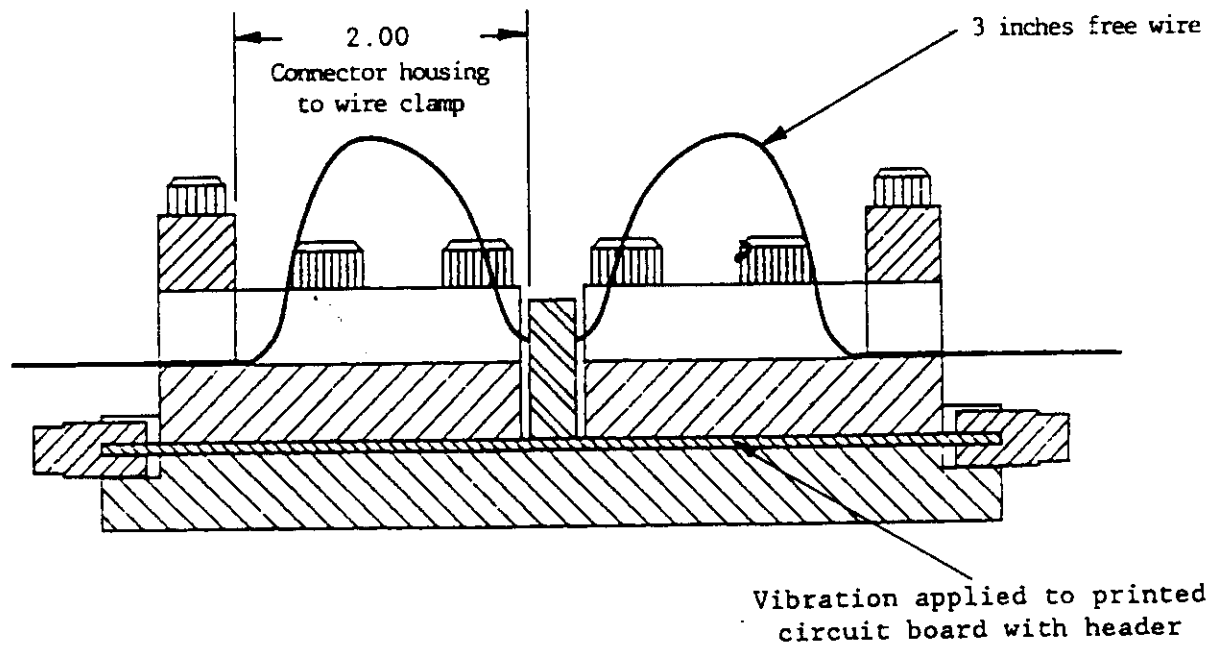
Figure 4 Vibration & Physical Shock Mounting Fixture
