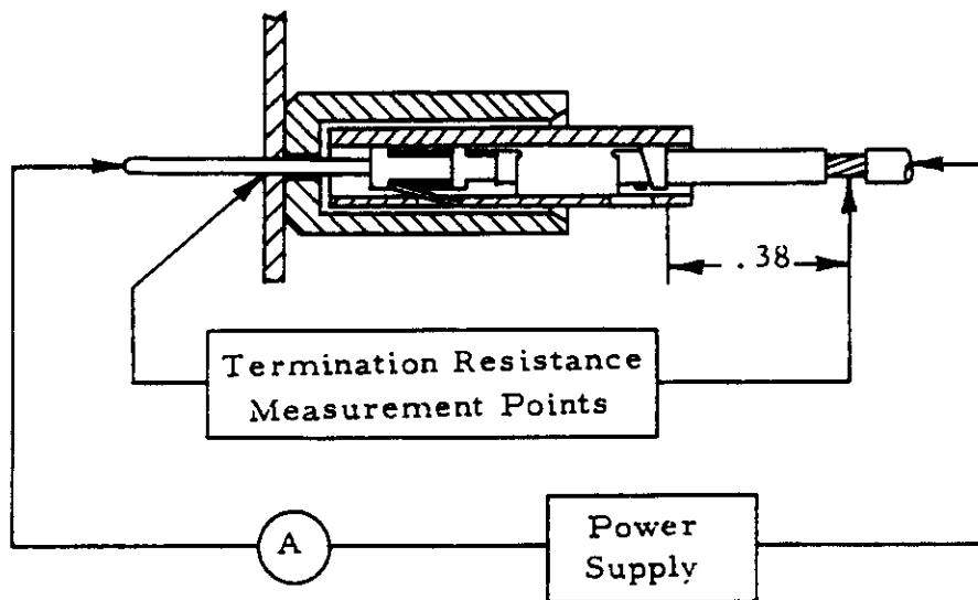
Figure 3 Termination Resistance Measurements
