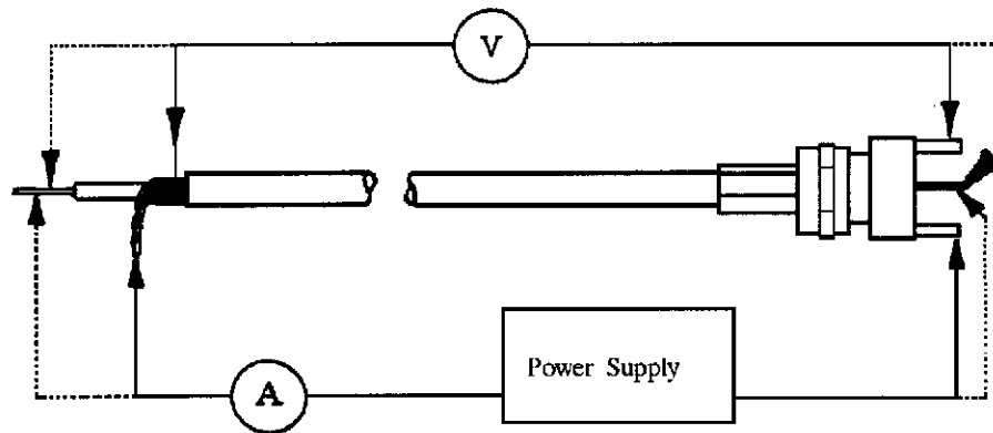
Figure 3 Dry Circuit Resistance Measurement Points
