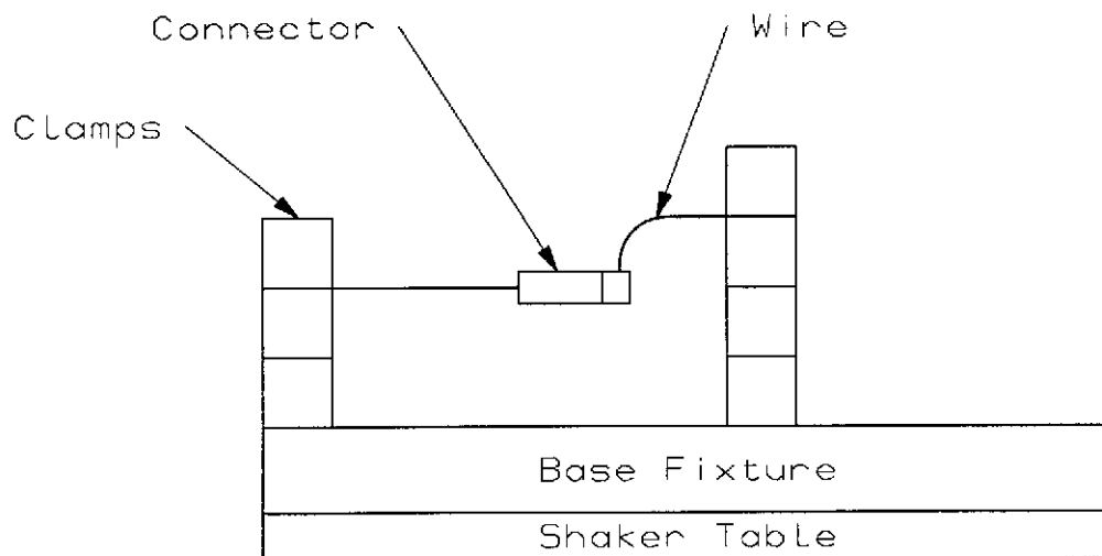
Wire-To-Wire Connector
