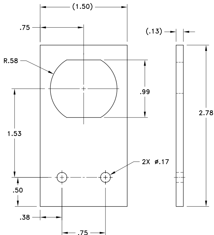
MOUNTING PATTERN
