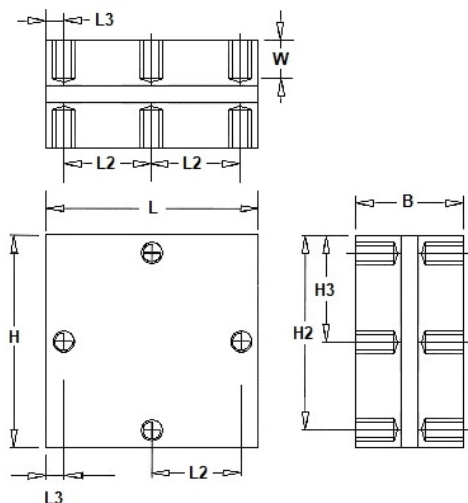
LEAD STYLE: 4TM6
