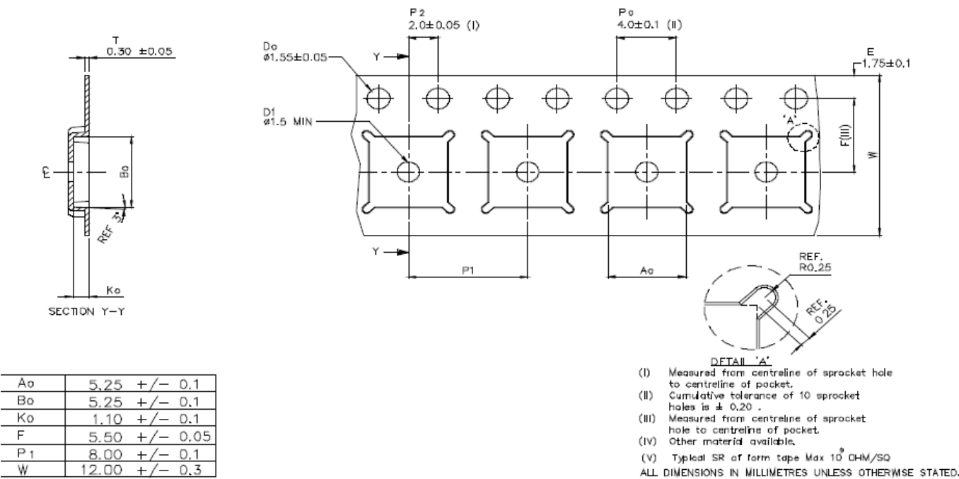
Figure 5-4: Tape & Reel Information
