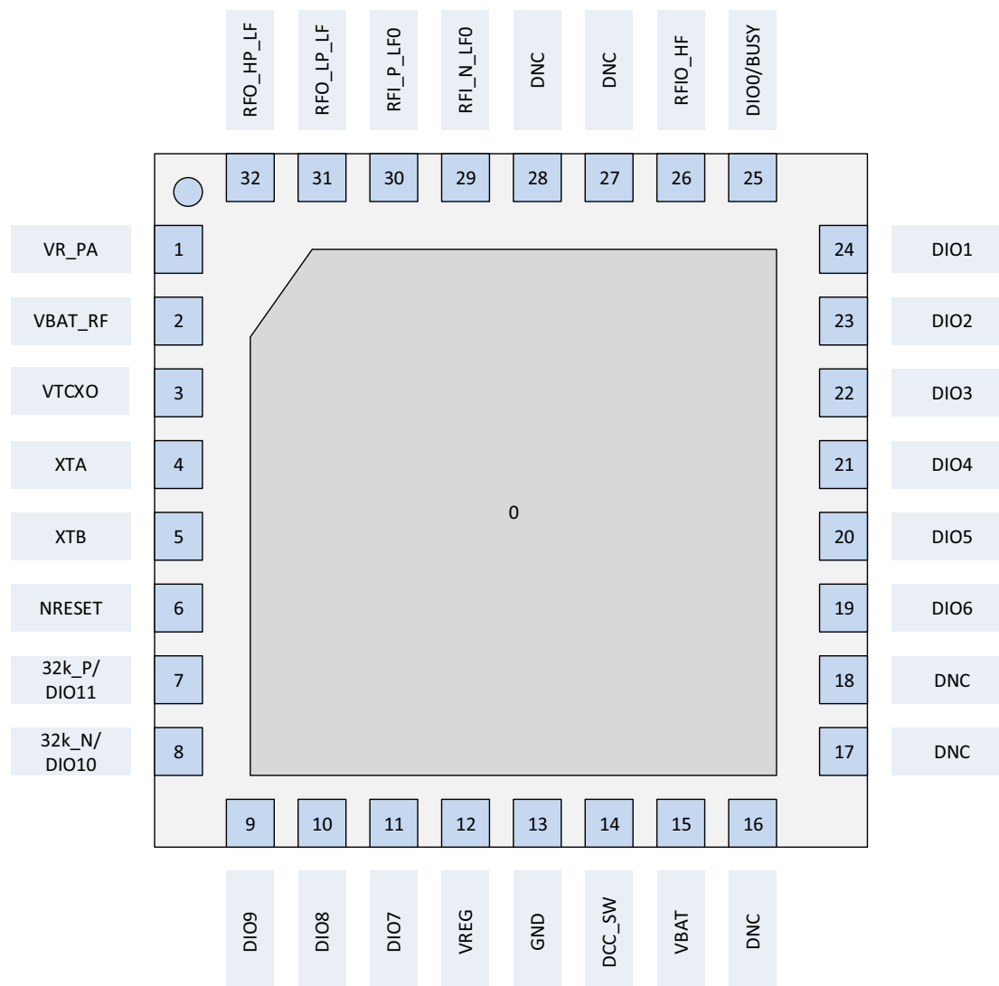
Figure 2-1: LR1121 Pinout
