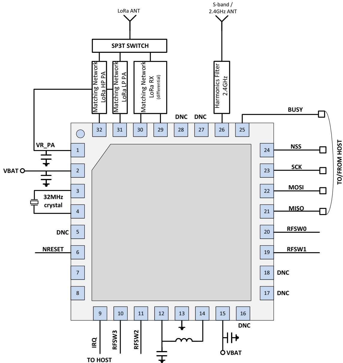
Figure 4-1: Multi-band EU/US LoRaWAN Using Sub-GHz PAs
