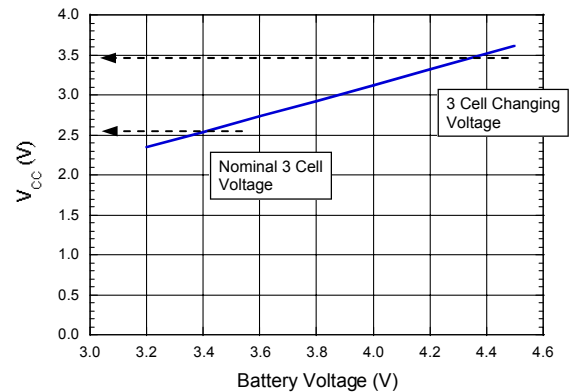
Figure 2. V_{CC} vs. 3 cell battery voltage with series dropping diode.
