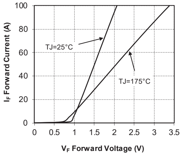
Figure 1-9. Forward Characteristics
