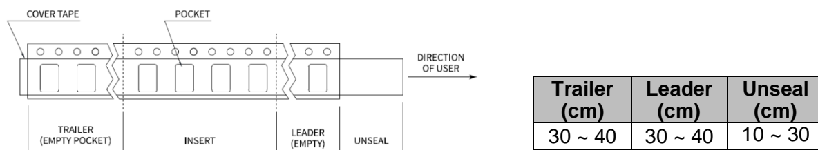
Figure 8 - Taping schedule.
