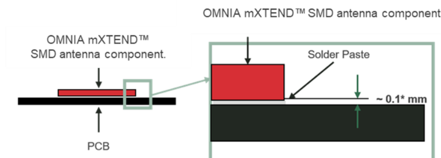
Figure 5 – Soldering Details.
