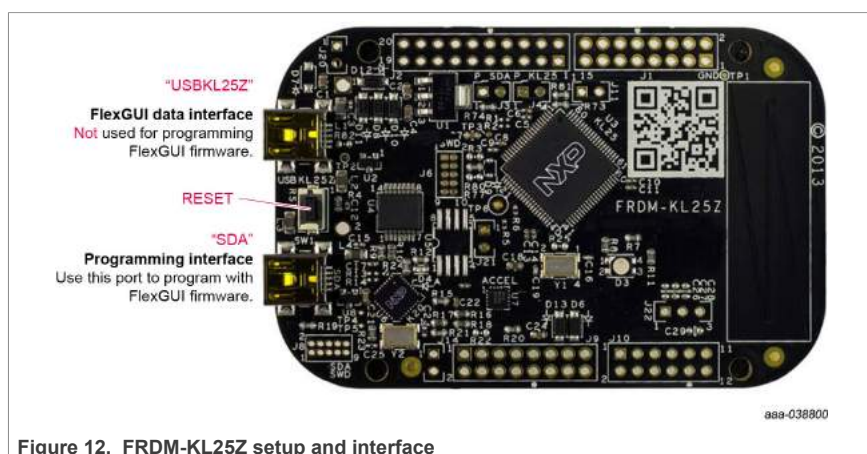
Figure 12. FRDM-KL25Z setup and interface
