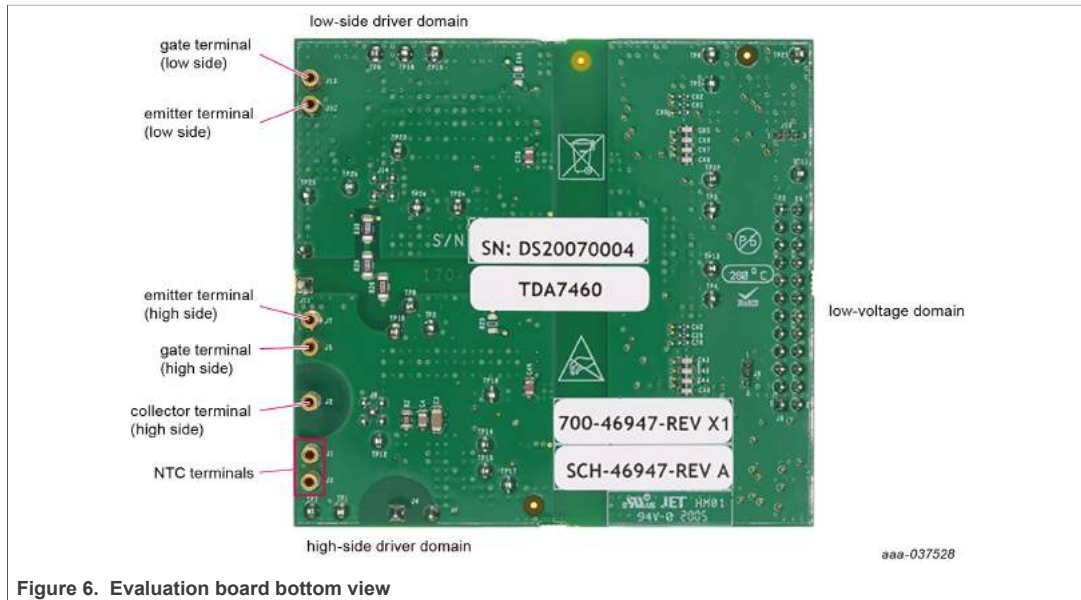
Figure 6. Evaluation board bottom view
