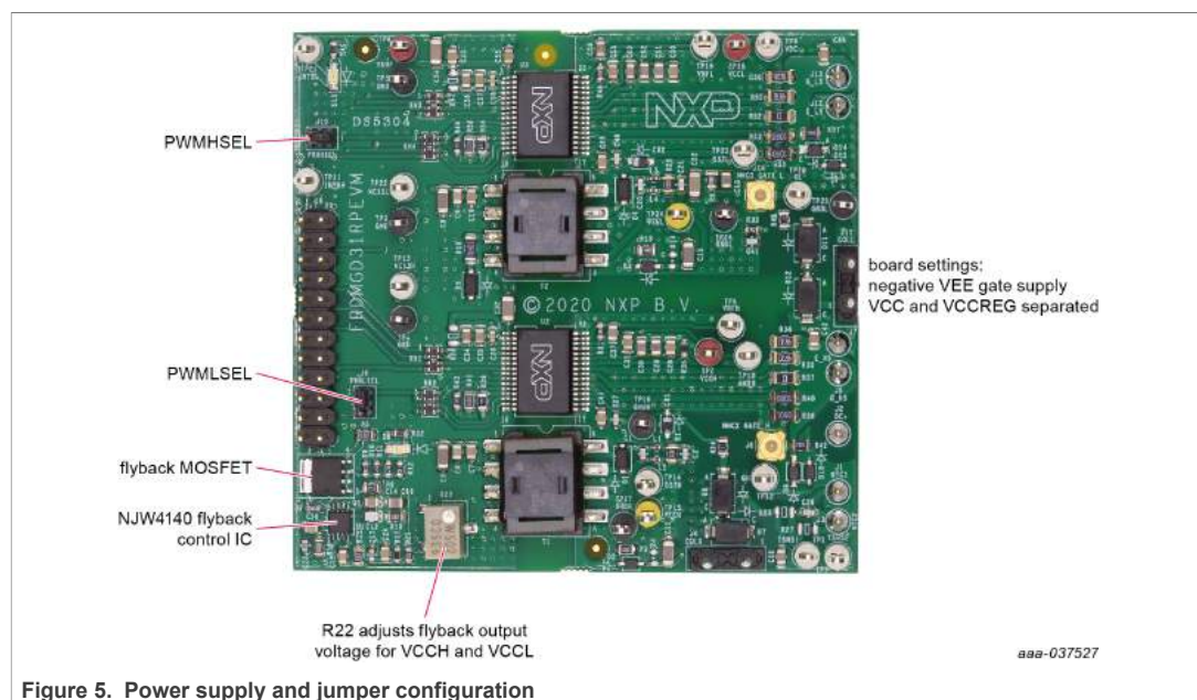
Figure 5. Power supply and jumper configuration
