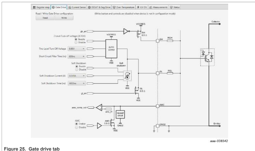
Figure 25. Gate drive tab
