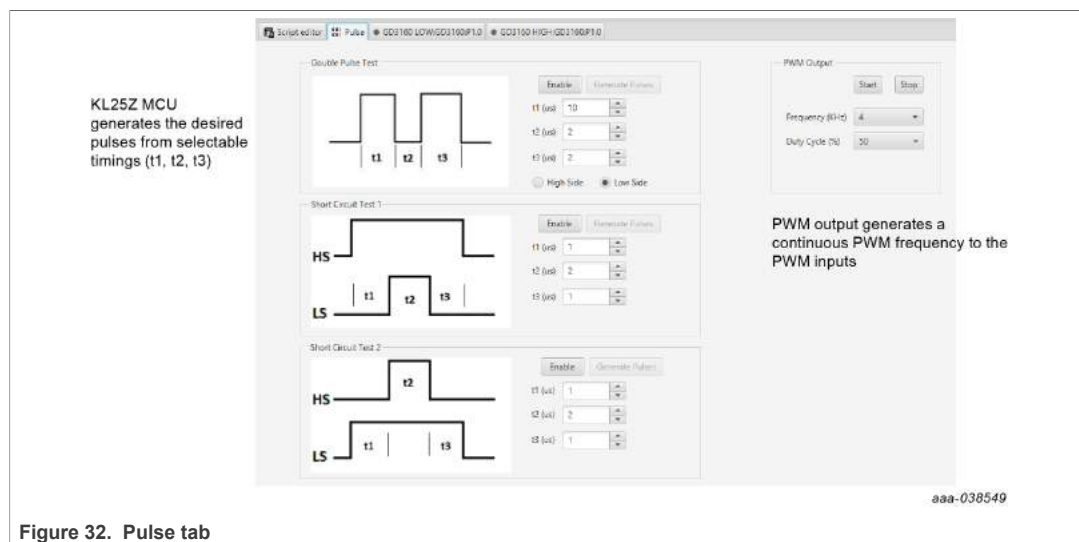
Figure 32. Pulse tab
