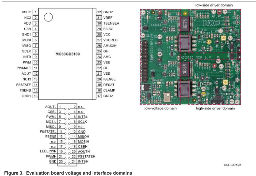
Figure 3. Evaluation board voltage and interface domains
