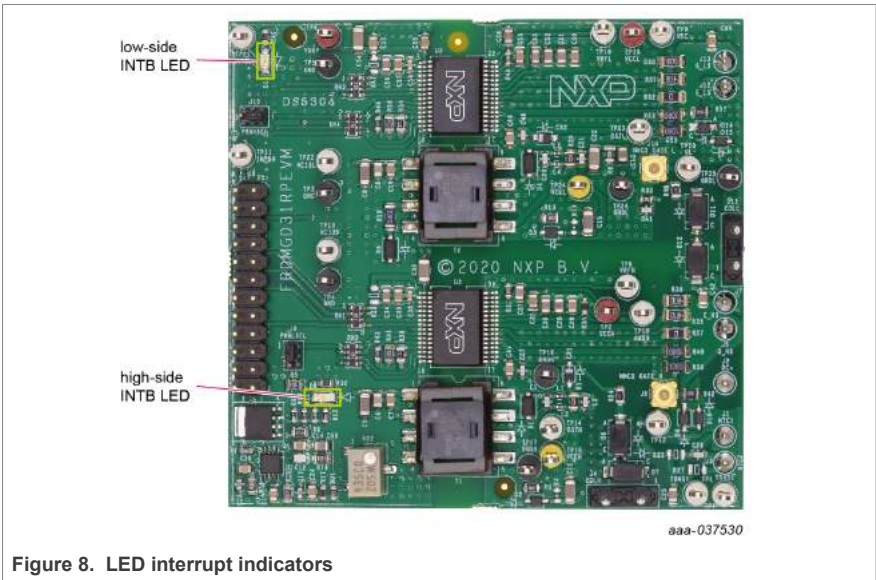
Figure 8. LED interrupt indicators
