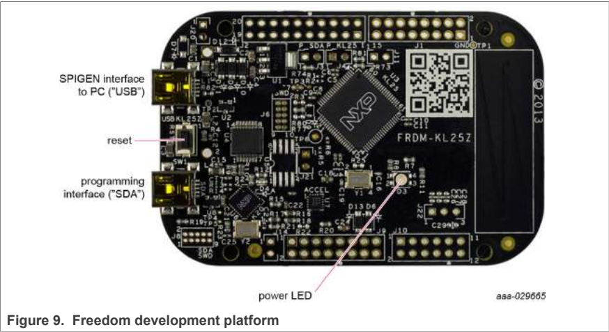
Figure 9. Freedom development platform
