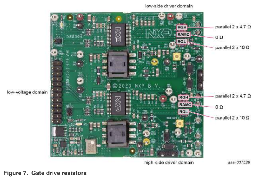
Figure 7. Gate drive resistors
