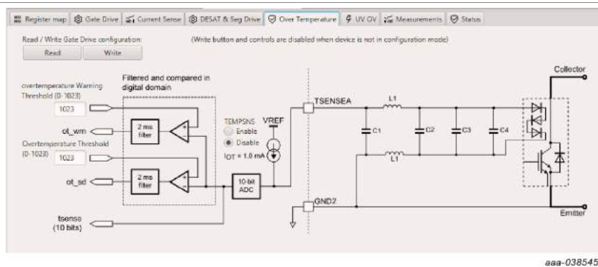
Figure 28. Overtemperature tab
