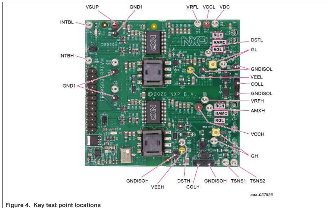
Figure 4. Key test point locations
