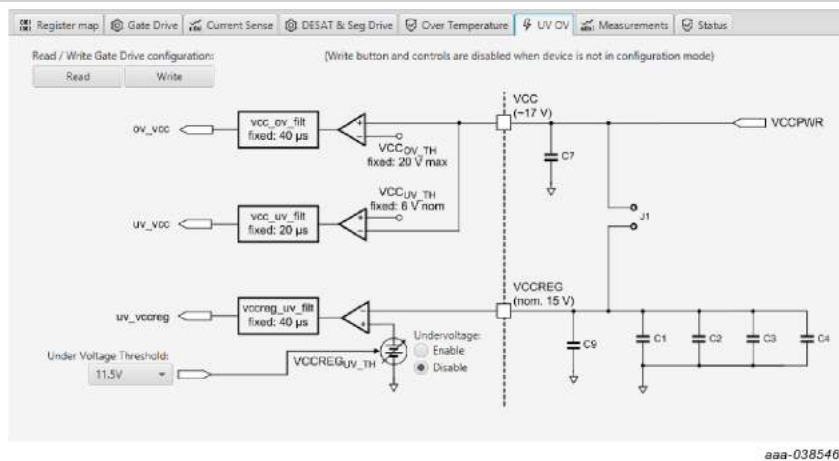
Figure 29. Undervoltage and overvoltage tab
