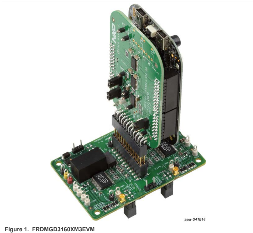
Figure 1. FRDMGD3160XM3EVM
