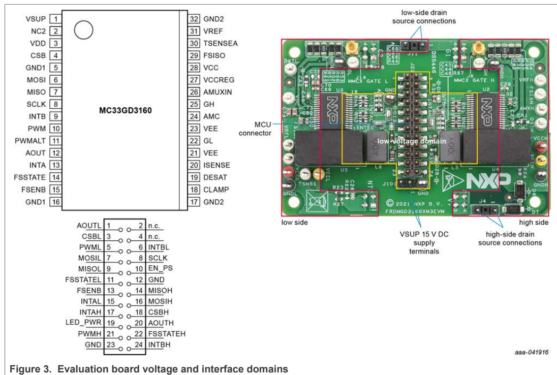
Figure 3. Evaluation board voltage and interface domains
