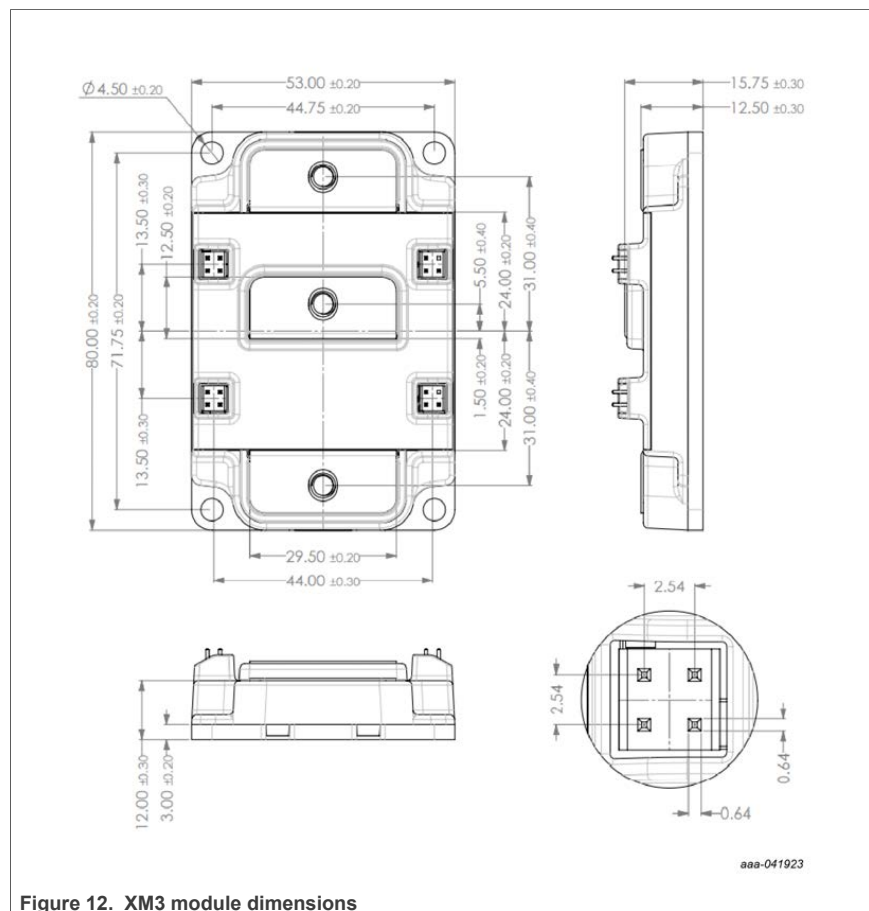
Figure 12. XM3 module dimensions
