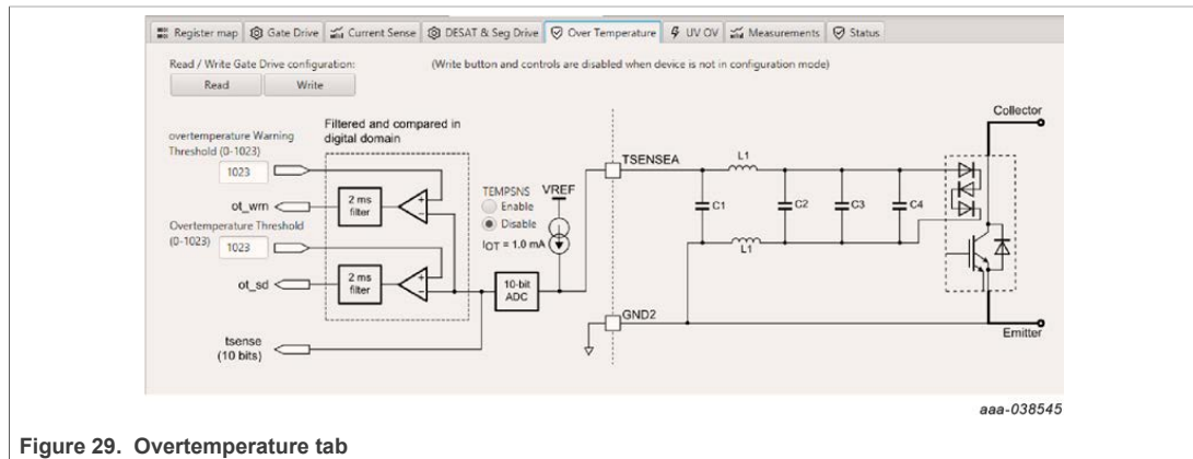
Figure 29. Overtemperature tab
