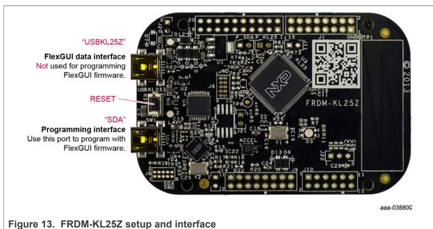
Figure 13. FRDM-KL25Z setup and interface
