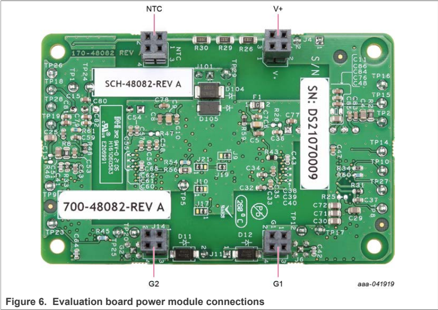
Figure 6. Evaluation board power module connections
