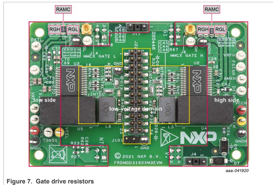
Figure 7. Gate drive resistors
