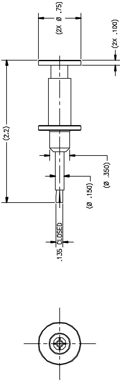
CLOSED POSITION
