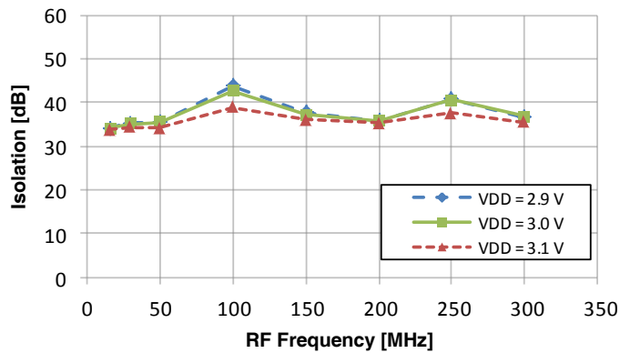
Figure 32. LO to IF Isolation vs V_{DD} (25 °C, –8 dBm LO Input, 325 MHz IF)
