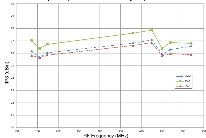
Figure 13. IIP3 vs Temperature (3.0V, –6 dBm LO Input, 109.65 MHz IF)
