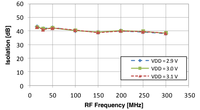
Figure 31. RF to IF Isolation vs V_{DD} (25 °C, –8 dBm LO Input, 325 MHz IF)
