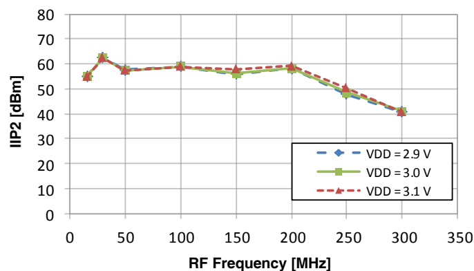
Figure 34. IIP2 vs V_{DD} (25 °C, –8 dBm LO Input, 325 MHz IF)
