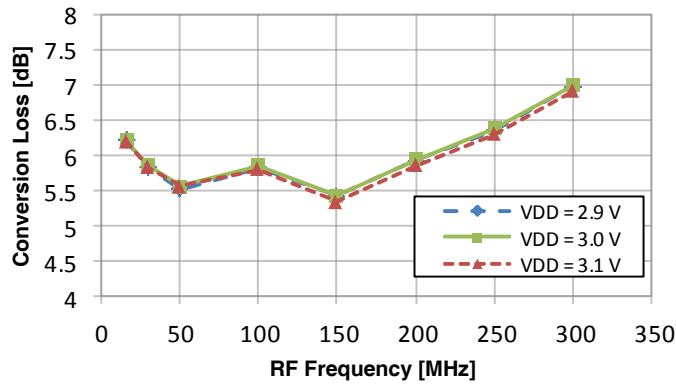
Figure 18. Conversion Loss vs V_{DD} (25 °C, –8 dBm LO Input, 7.5 MHz IF)
