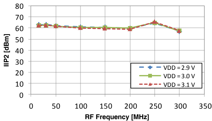
Figure 22. IIP2 vs V_{DD} (25 °C, –8 dBm LO Input, 7.5 MHz IF)
