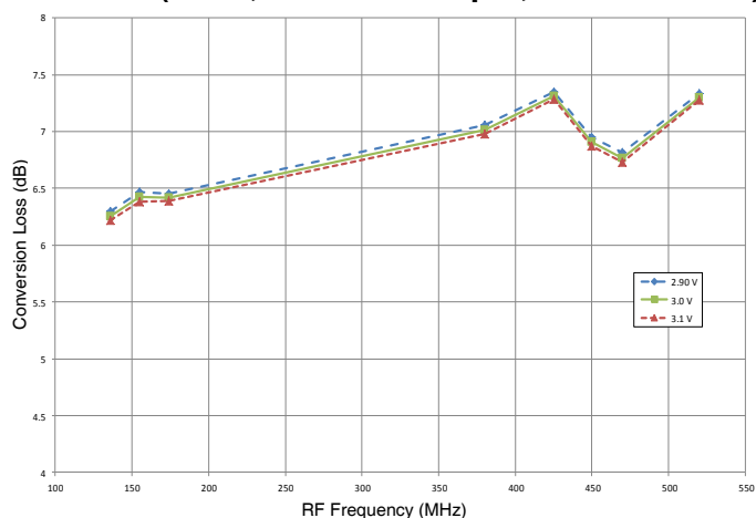
Figure 4. Conversion Loss vs Voltage (25 °C, -6 dBm LO Input, 109.65 MHz IF)
