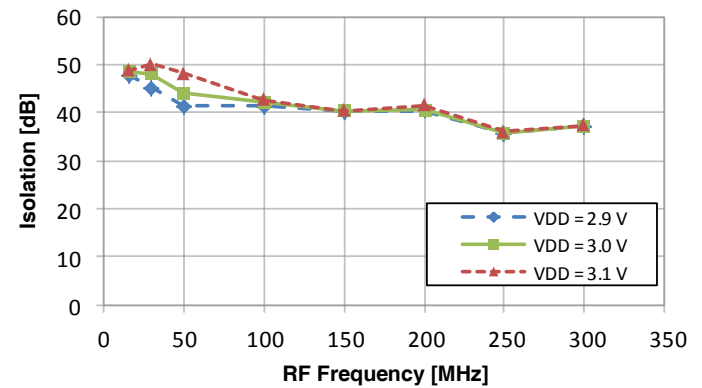
Figure 33. LO to RF Isolation vs V_{DD} (25 °C, –8 dBm LO Input, 325 MHz IF)
