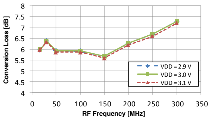
Figure 24. Conversion Loss vs V_{DD} (25 °C, -8 dBm LO Input, 110 MHz IF)
