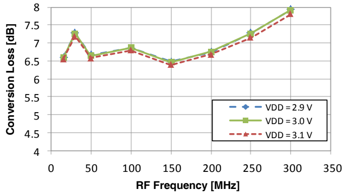
Figure 30. Conversion Loss vs V_{DD} (25 °C, –8 dBm LO Input, 325 MHz IF)
