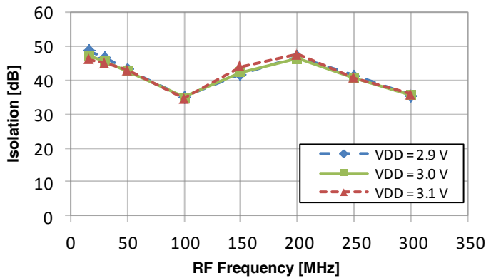
Figure 20. LO to IF Isolation vs V_{DD} (25 °C, –8 dBm LO Input, 7.5 MHz IF)
