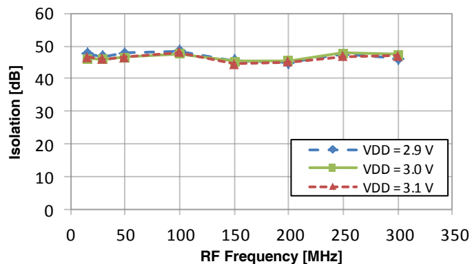
Figure 25. RF to IF Isolation vs V_{DD} (25 °C, -8 dBm LO Input, 110 MHz IF)
