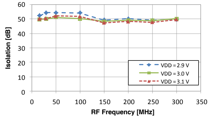
Figure 19. RF to IF Isolation vs V_{DD} (25 °C, –8 dBm LO Input, 7.5 MHz IF)
