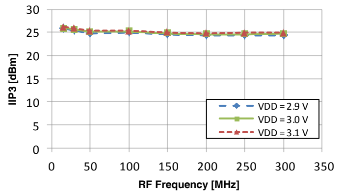
Figure 23. IIP3 vs V_{DD} (25 °C, –8 dBm LO Input, 7.5 MHz IF)
