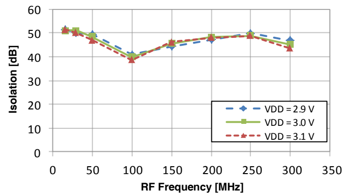
Figure 21. LO to RF Isolation vs V_{DD} (25 °C, –8 dBm LO Input, 7.5 MHz IF)
