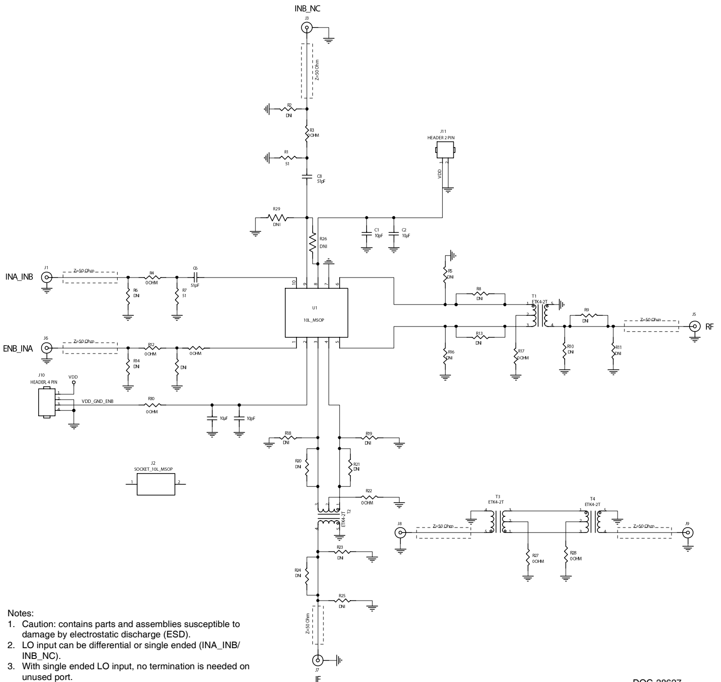
Figure 45. Evaluation Board Schematic
