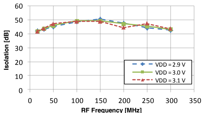
Figure 27. LO to RF Isolation vs V_{DD} (25 °C, -8 dBm LO Input, 110 MHz IF)
