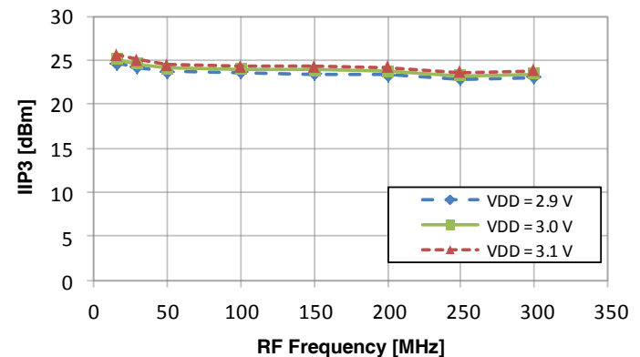
Figure 35. IIP3 vs V_{DD} (25 °C, –8 dBm LO Input, 325 MHz IF)
