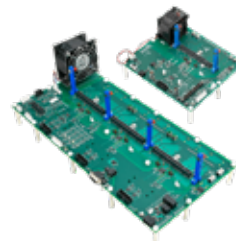
SpeedVal™ 3-Phase Motherboard
