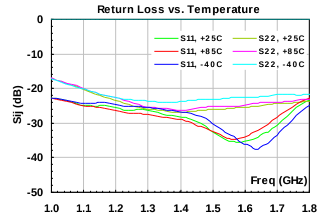
FIG. 6 Return Loss vs. Temperature
