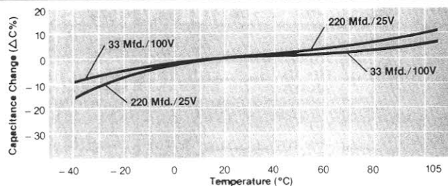
DISSIPATION FACTOR ( \tan \delta ) vs. TEMPERATURE
