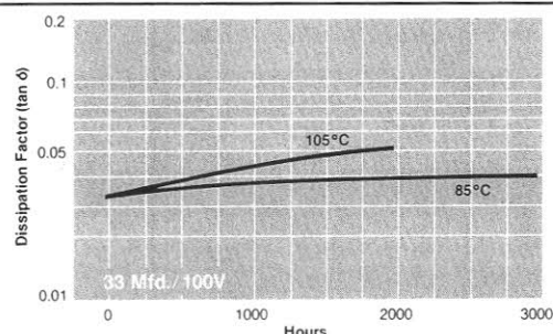
DISSIPATION FACTOR ( \tan \delta ) vs. TIME
