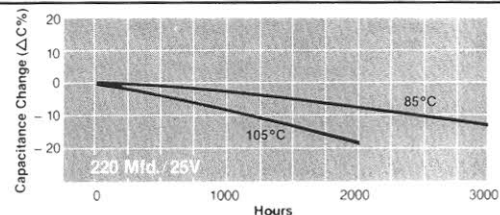
CAPACITANCE CHANGE ( \Delta C\% ) vs. TIME
