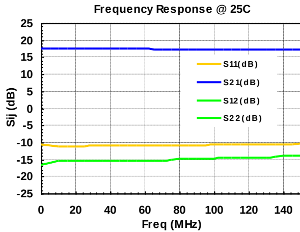
FIG. 1 Small signal performance.
