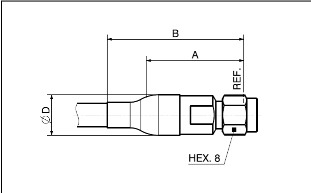
Connector 11_SMA (straight male)
