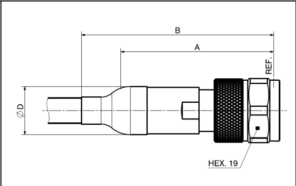
Connector 11_N (straight male)
