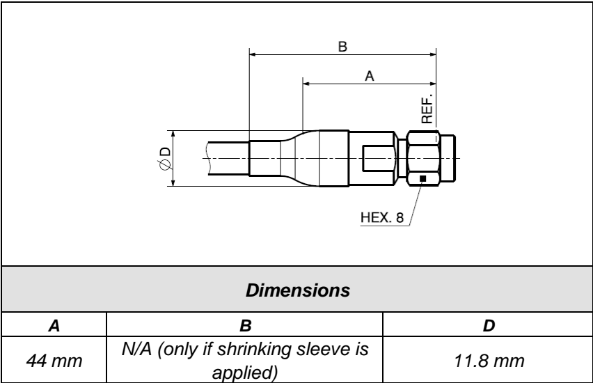
Connector 11_SMA (straight male)
