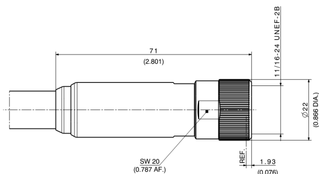
Figure 1: 35 VM (3.5 mm ruggedized PORT female)
