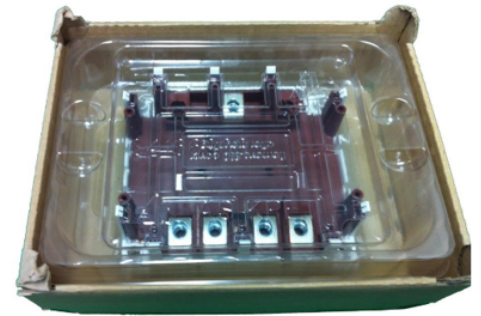
Figure 1 Current carton box packaging and plastic blister for SKiM®4 currently delivered without pre-applied TIM
