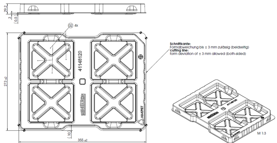
Figure 2: New Tray-4 fold
