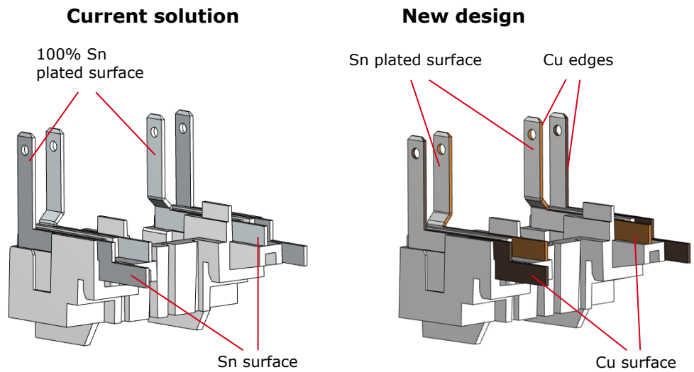
Auxiliary contacts with fixing base inside the housing
