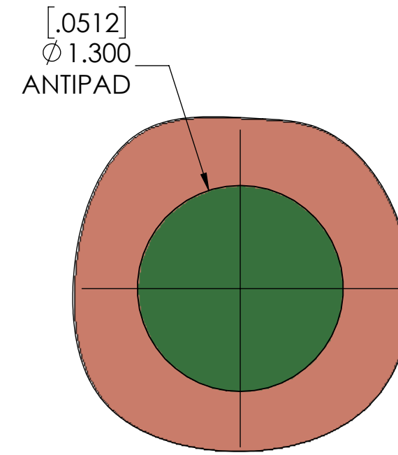
DETAIL B SCALE 30:1 LAYER 3 (Cu) VIAS NOT SHOWN FOR CLARITY
