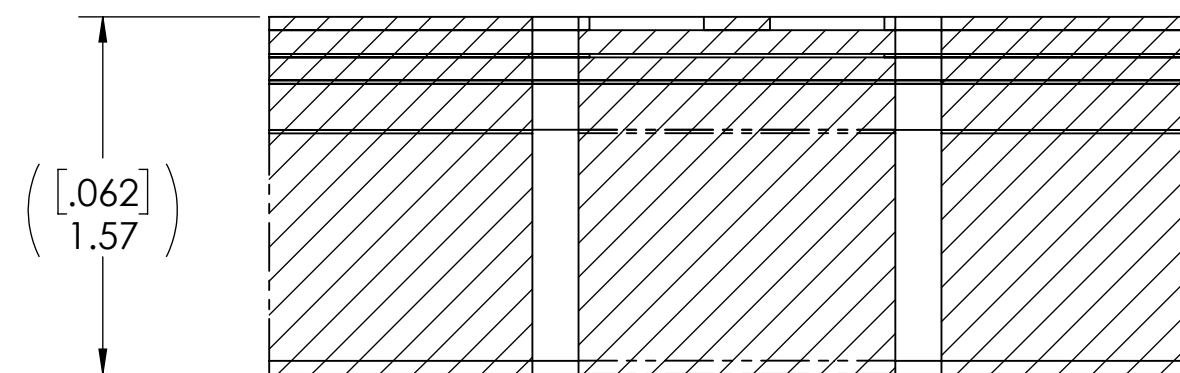
SECTION C-C SCALE 30 : 1 PCB LAYER DEFINITION
