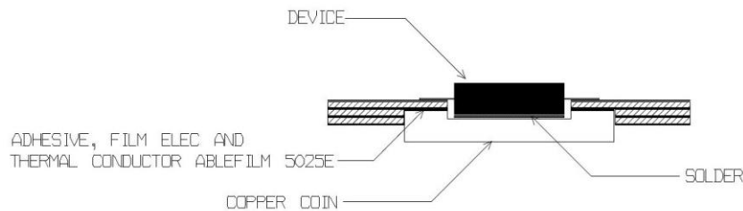
DEVICE SOLDERING DETAIL
