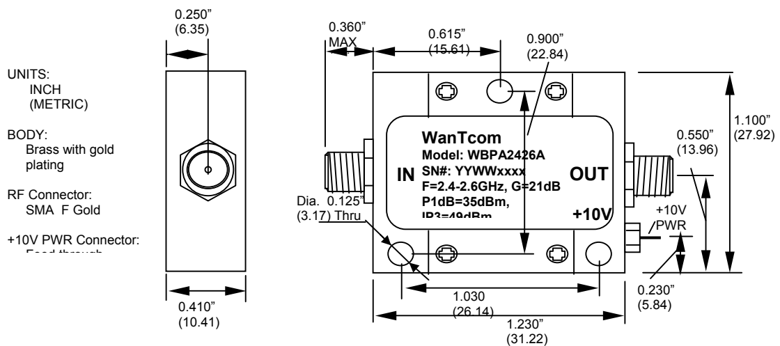
FIG. 6 WBPA2426A outline
