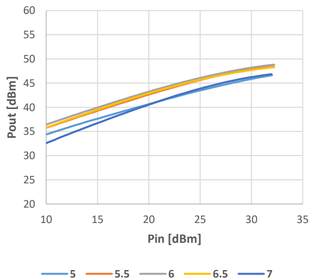
[32V] Pout vs. Pin
