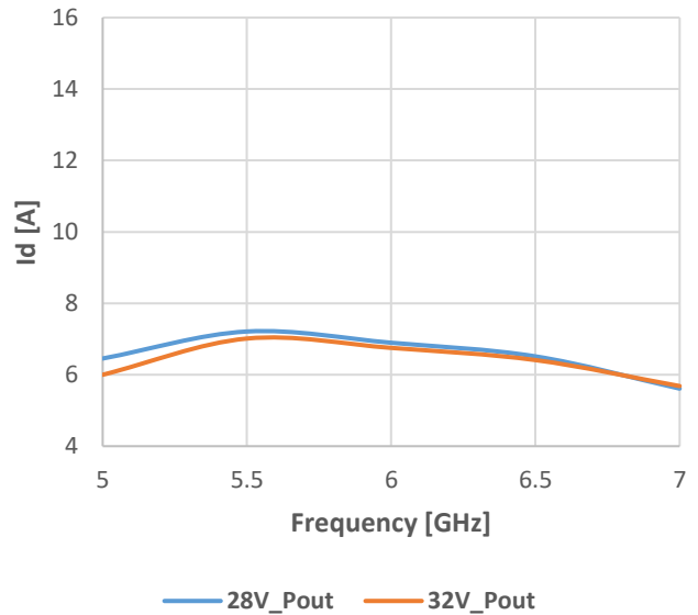
Id vs. Frequency
