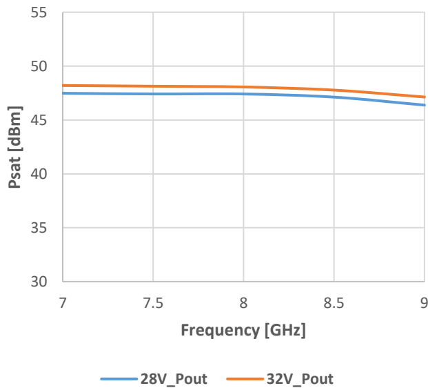
Psat vs. Frequency
