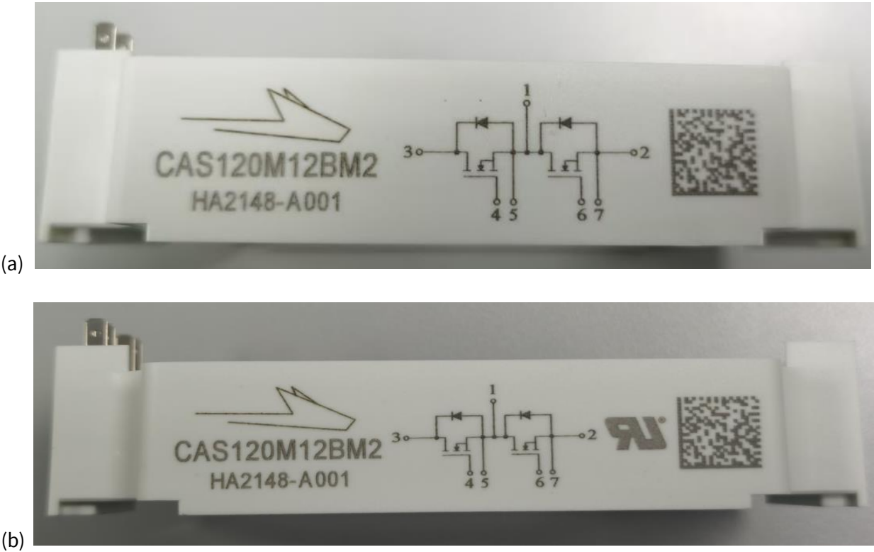
Figure 1. (a) Current marking with no UL logo (b) New laser marking on the Power Modules with UL registered logo.
