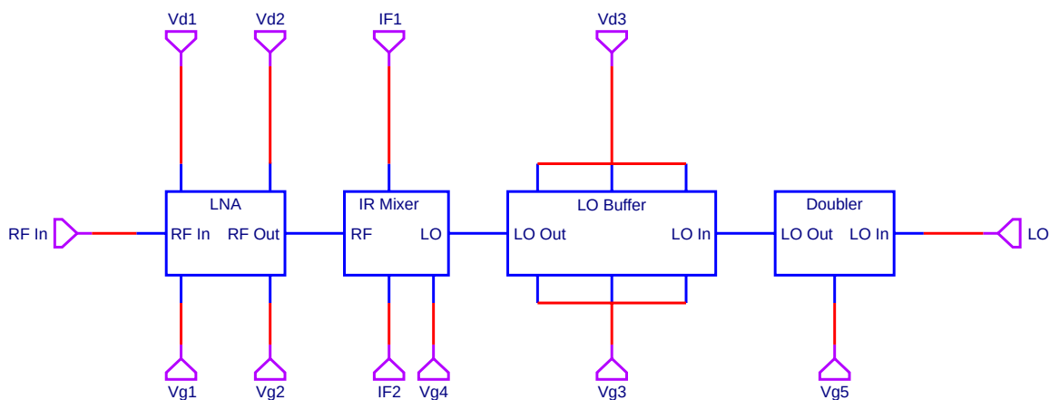
Block Diagram
