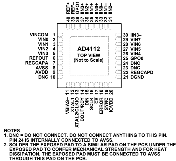
Figure 4. Pin Configuration
