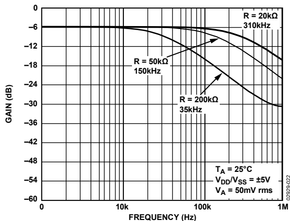
Figure 24. -3 dB Bandwidth
