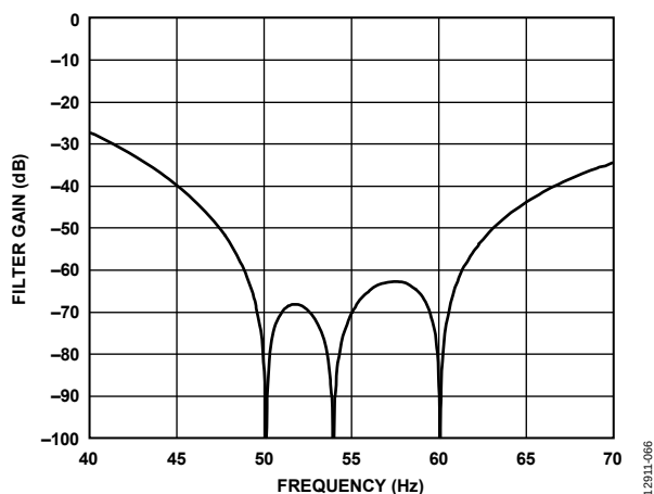
Figure 63. 25 SPS ODR, 40 ms Settling Time at 50 Hz/60 Hz
