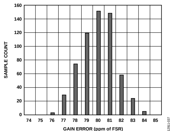
Figure 33. Gain Error Distribution Histogram (All Input Buffers Disabled, 647 Units)
