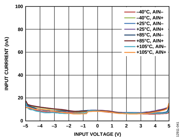
Figure 40. Analog Input Current vs. Input Voltage ( V_{CM} = 2.5\text{ V} )
