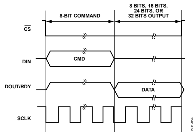
Figure 44. Reading from a Register (8-Bit Command with Register Address Followed by Data of 8, 16, or 24 Bits; Data Length on DOUT Is Dependent on the Register Selected)
