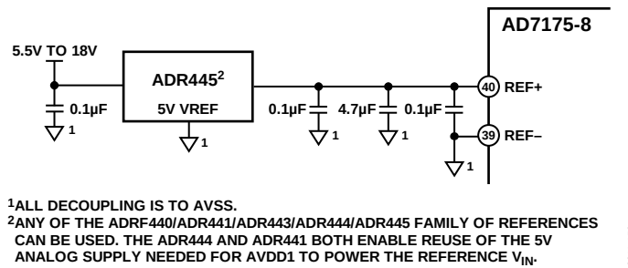
Figure 52. External Reference ADR445 Connected to the AD7175-8 Reference Pins
