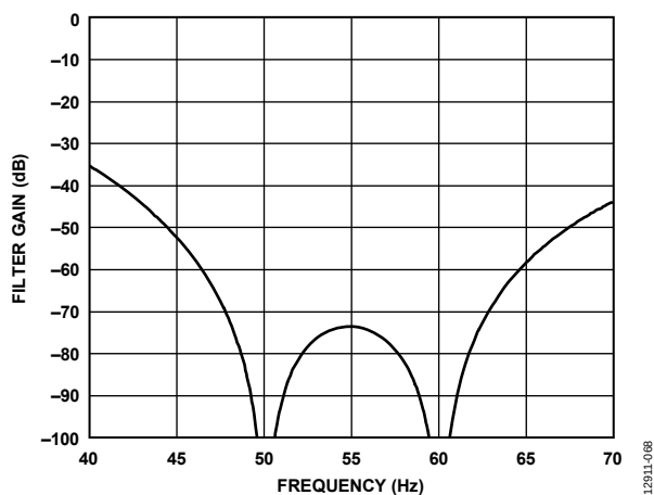
Figure 64. 20 SPS ODR, 50 ms Settling Time at 50 Hz/60 Hz
