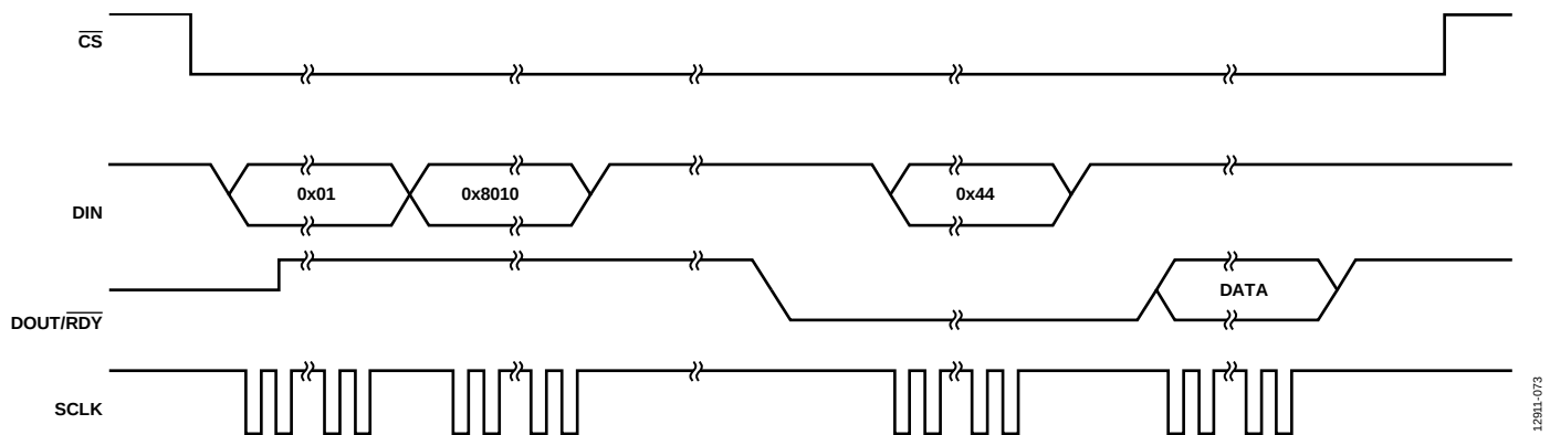
Figure 69. Single Conversion Mode
