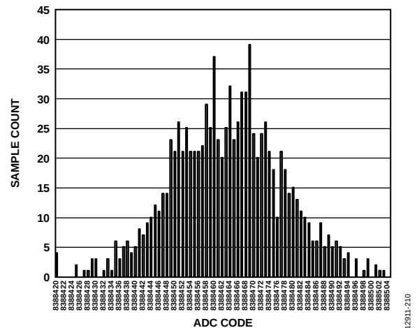
Figure 10. Histogram (Analog Input Buffers Disabled, V_{REF} = 5\text{ V} , Output Data Rate = 250 kSPS)
