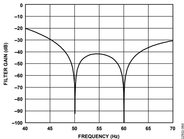
Figure 62. 27.27 SPS ODR, 36.67 ms Settling Time at 50 Hz/60 Hz
