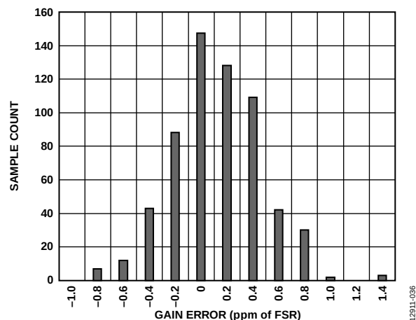
Figure 32. Gain Error Distribution Histogram (All Input Buffers Enabled, 611 Units)
