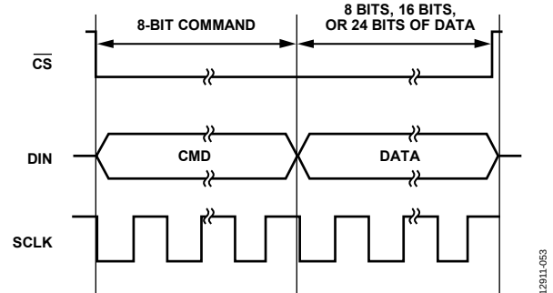
Figure 43. Writing to a Register (8-Bit Command with Register Address Followed by Data of 8, 16, or 24 Bits; Data Length on DIN Is Dependent on the Register Selected)
