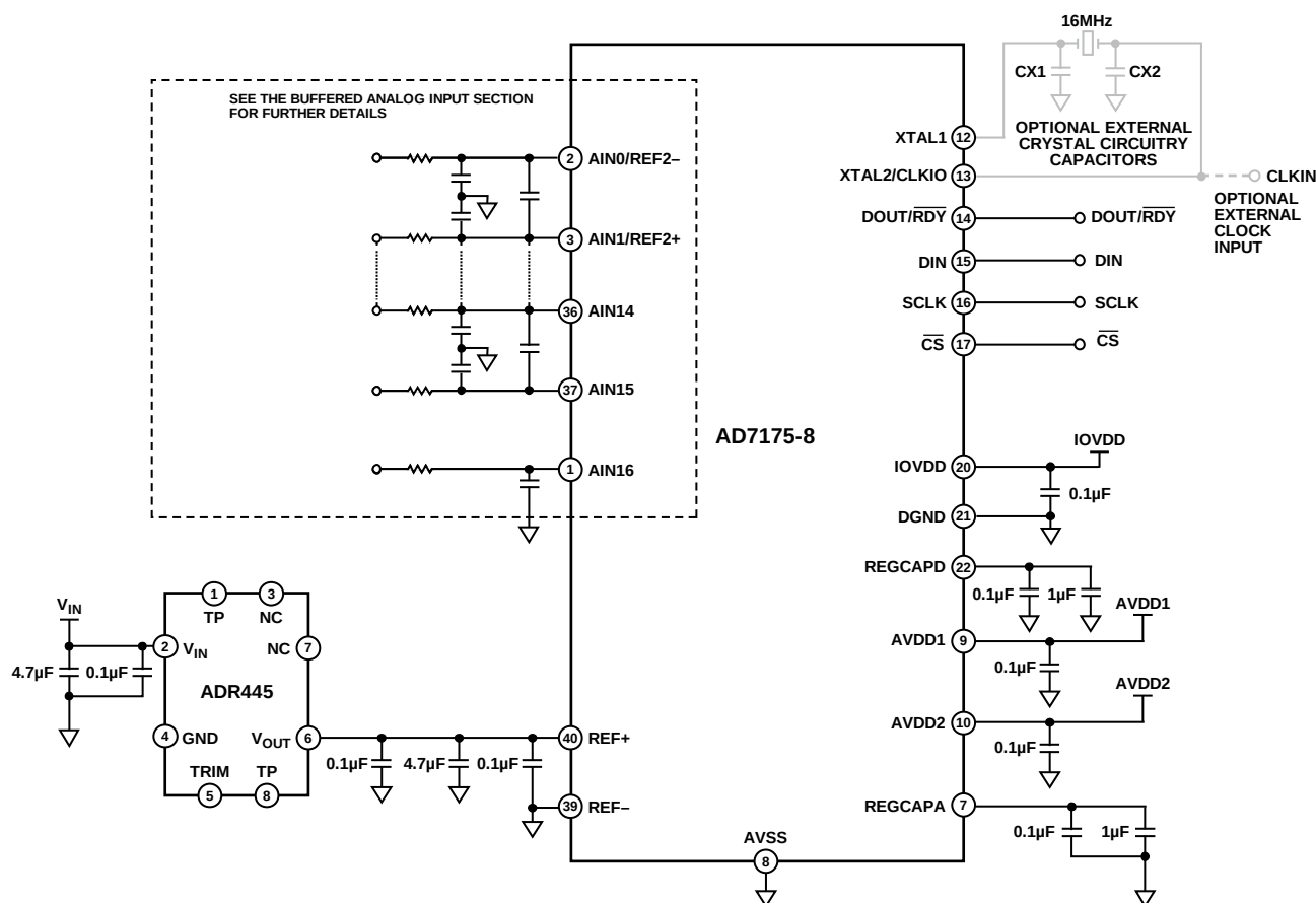
Figure 41. Typical Connection Diagram
