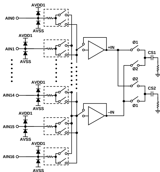
Figure 51. Simplified Analog Input Circuit
