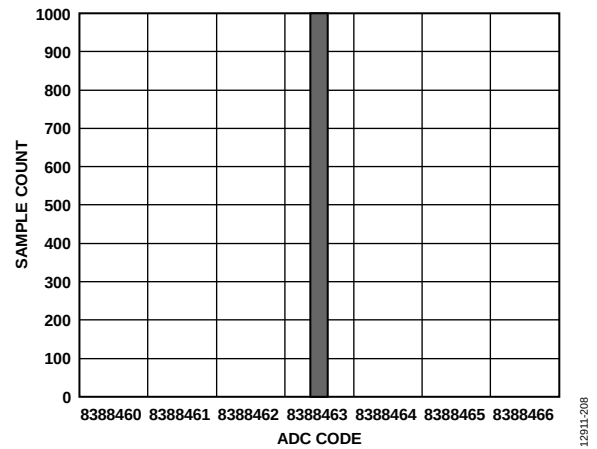
Figure 8. Histogram (Analog Input Buffers Disabled, V_{REF} = 5\text{ V} , Output Data Rate = 5 SPS)
