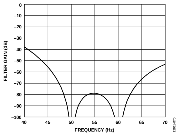
Figure 66. 16.667 SPS ODR, 60 ms Settling Time at 50 Hz/60 Hz
