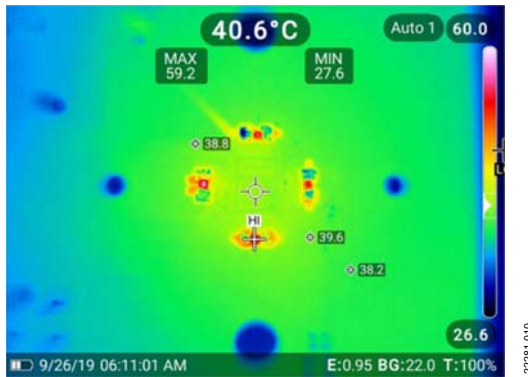
Figure 9. Infrared Image of the CN-0537 Heating Resistors
