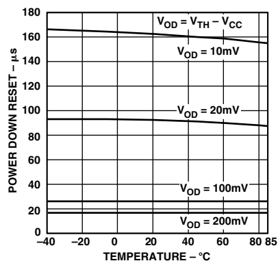
TPC 4. Power-Down Reset Delay vs. Temperature ADM809-5S
