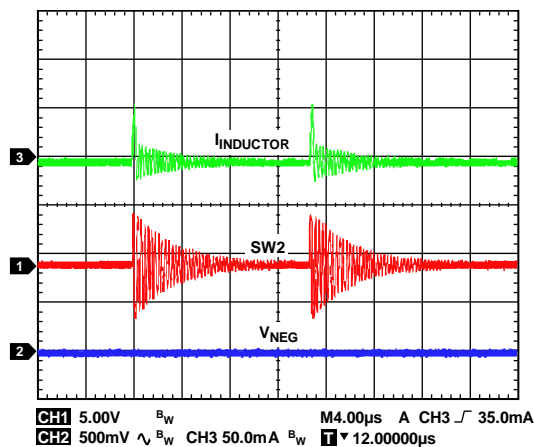
Figure 36. Inverting Regulator Skip Mode Operation Showing Inductor Current ( I_{INDUCTOR} ), Switch Node Voltage, and Output Ripple, V_{IN} = 5 V, V_{NEG} = -5 V, I_{LOAD2} = 0 mA, f_{SW} = 2.4 MHz, T_A = 25^\circ\text{C}
