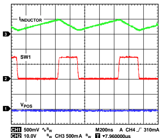
Figure 35. Boost Regulator Continuous Conduction Mode Operation Showing Inductor Current ( I_{INDUCTOR} ), Switch Node Voltage, and Output Ripple, V_{IN} = 5 V, V_{POS} = 15 V, I_{LOAD1} = 90 mA, f_{SW} = 2.4 MHz, T_A = 25^\circ\text{C}
