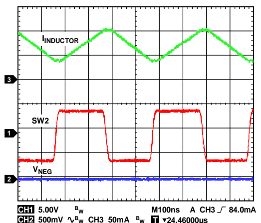
Figure 38. Inverting Regulator Continuous Conduction Mode Operation Showing Inductor Current ( I_{INDUCTOR} ), Switch Node Voltage, and Output Ripple, V_{IN} = 5 V, V_{NEG} = -5 V, I_{LOAD2} = 35 mA, f_{SW} = 2.4 MHz, T_A = 25^\circ\text{C}
