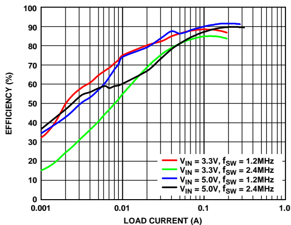
Figure 10. Efficiency vs. Load Current for Boost Regulator, V_{POS} = 15\text{ V} , T_A = 25^\circ\text{C}
