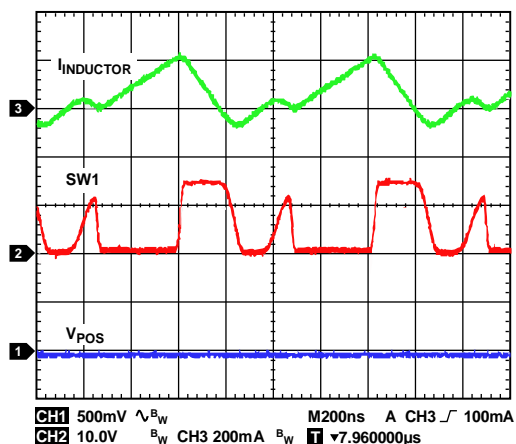
Figure 34. Boost Regulator Discontinuous Conduction Mode Operation Showing Inductor Current ( I_{INDUCTOR} ), Switch Node Voltage, and Output Ripple, V_{IN} = 5 V, V_{POS} = 15 V, I_{LOAD1} = 6 mA, f_{SW} = 2.4 MHz, T_A = 25^\circ\text{C}
