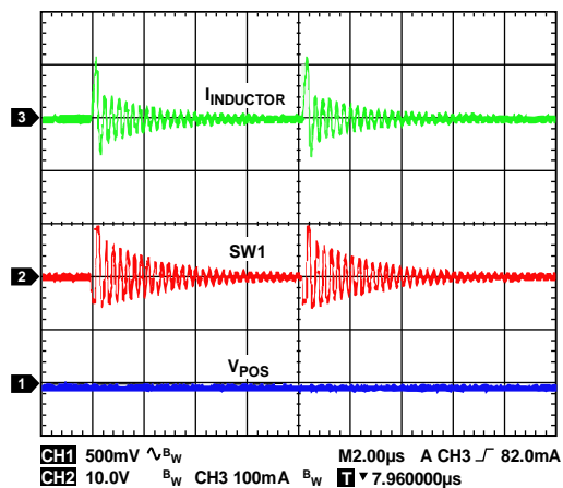
Figure 33. Boost Regulator Skip Mode Operation Showing Inductor Current ( I_{INDUCTOR} ), Switch Node Voltage, and Output Ripple, V_{IN} = 12 V, V_{POS} = 15 V, I_{LOAD1} = 4 mA, f_{SW} = 2.4 MHz, T_A = 25^\circ\text{C}
