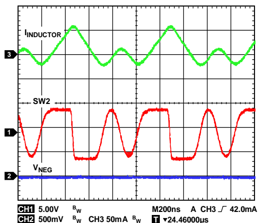
Figure 37. Inverting Regulator Discontinuous Conduction Mode Operation Showing Inductor Current ( I_{INDUCTOR} ), Switch Node Voltage, and Output Ripple, V_{IN} = 5 V, V_{NEG} = -5 V, I_{LOAD2} = 6 mA, f_{SW} = 2.4 MHz, T_A = 25^\circ\text{C}
