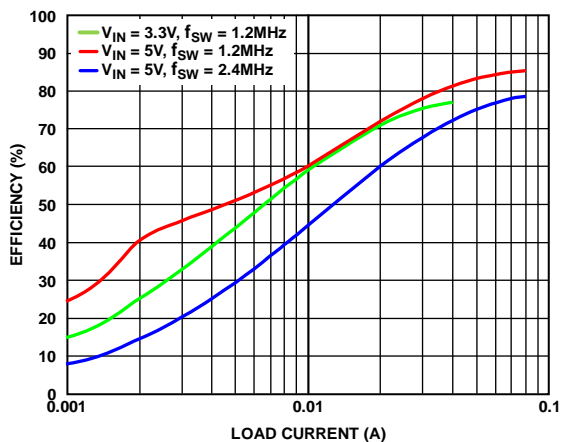
Figure 11. Efficiency vs. Load Current for Boost Regulator, V_{POS} = 35\text{ V} , T_A = 25^\circ\text{C}
