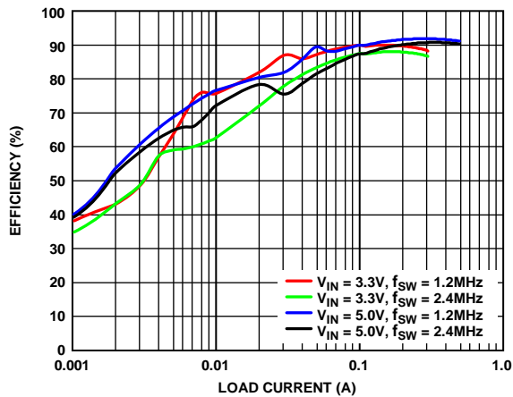
Figure 9. Efficiency vs. Load Current for Boost Regulator, V_{POS} = 9\text{ V} , T_A = 25^\circ\text{C}
