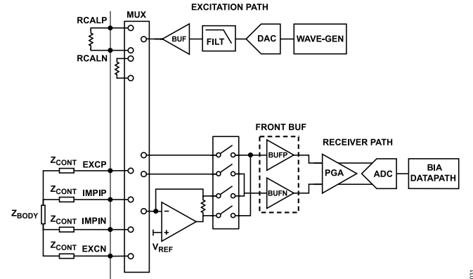
Figure 32. BIA Channel Block Diagram ( Z_{CONT} Is Contact Impedance and Z_{BODY} Is Human Body Impedance)
