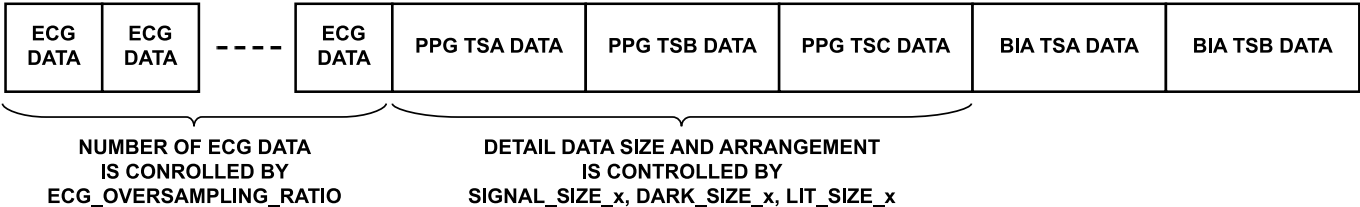
Figure 36. Example of Data Arrangement in the FIFO (TSA Is Time Slot A, TSB Is Time Slot B, and TSC Is Time Slot C)
