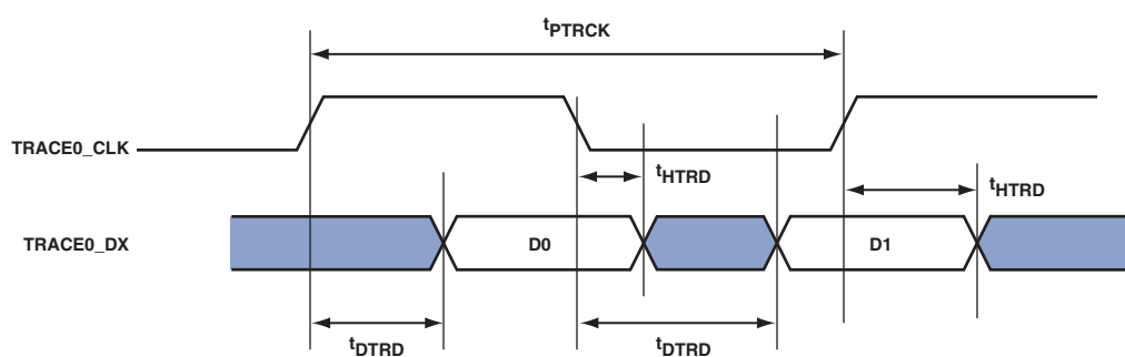
Figure 37. Trace Timing
