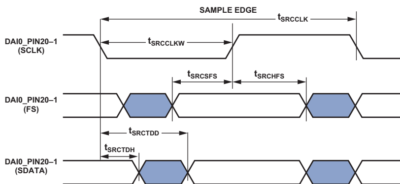
Figure 17. ASRC Serial Output Port Timing
