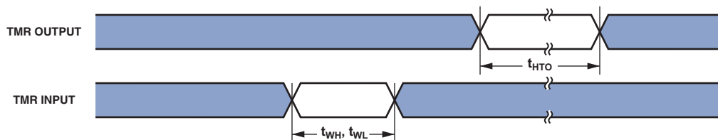
Figure 28. Timer Cycle Timing
