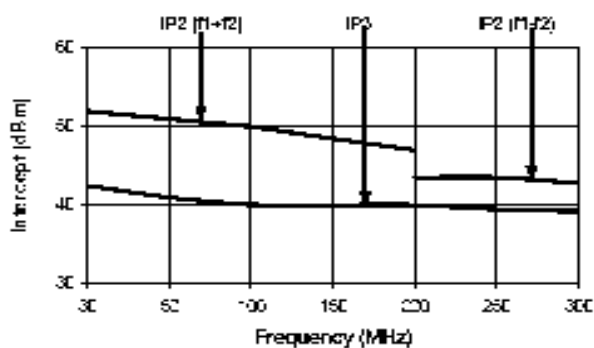
Intermodulation Intercept
