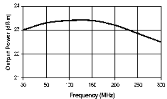
1 dB Compression
