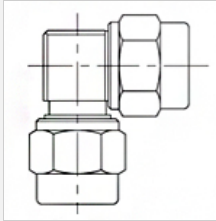
Right angle SMA plug - SMA plug Part no. 29212-2
