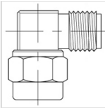
Right angle SMA plug - SMA jack Part no. 29212-1
