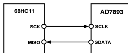
Figure 7. AD7893 to 68HC11 Interface
