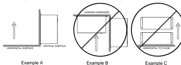
Figure 3-1: M3713DM Mounting Orientation
