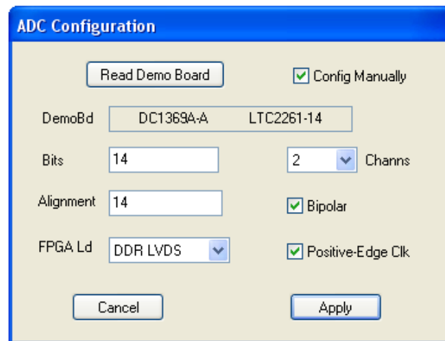
Figure 2: ADC configuration
