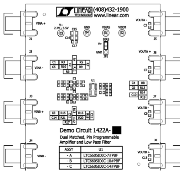
Figure 1. The DC1422 Top Silk Screen
