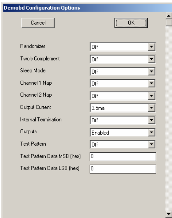
Figure 4: Demobd Configuration Options.
