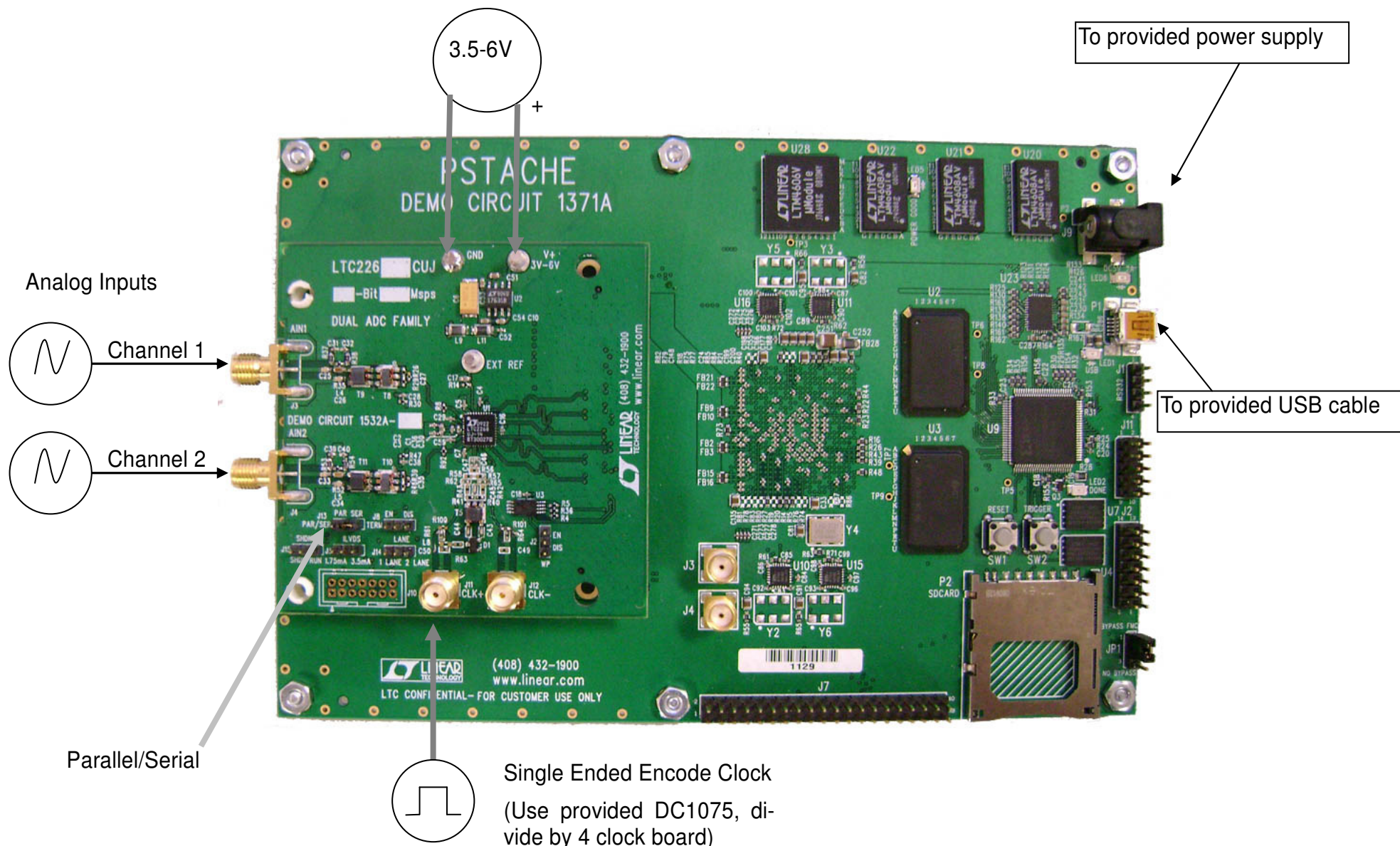
Figure 1. DC1532 Setup (zoom for detail)
