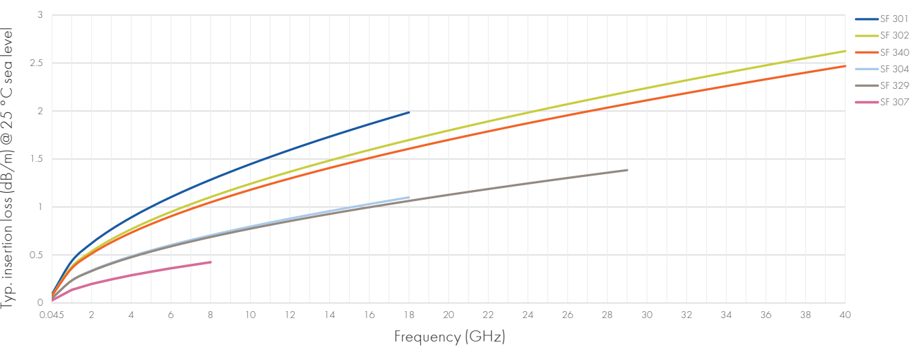
Attenuation (typical values at +25 °C ambient temperature)
