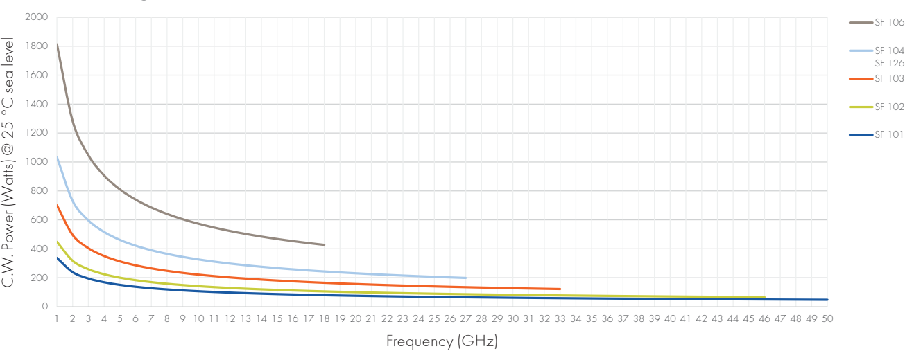
Power handling (maximum values at 25 °C ambient temperature and sea level)
