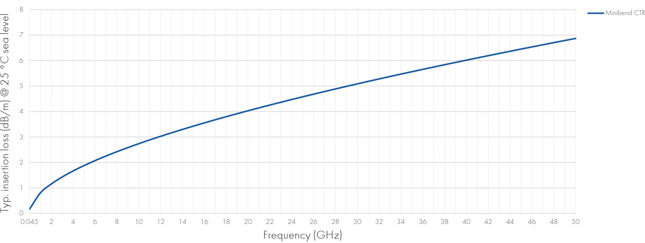
Attenuation (nominal values at +25 °C ambient temperature)
