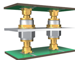
Board-to-board through a panel
