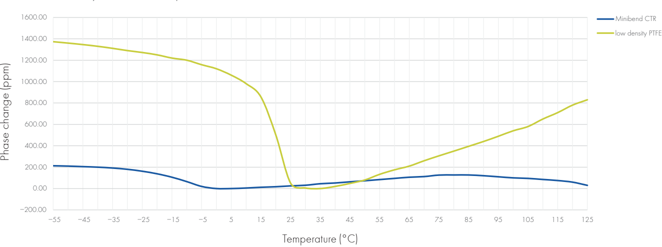
Phase stability versus temperature
