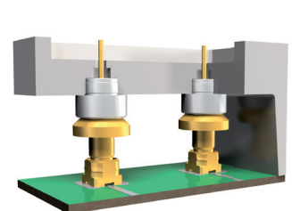
Board-to-panel connection (filter)
