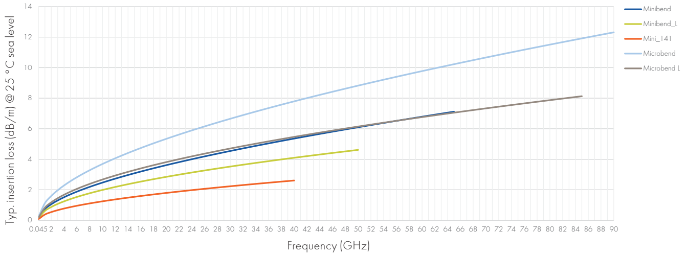
Attenuation (nominal values at +25 °C ambient temperature)
