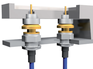
Panel-to-panel connection
