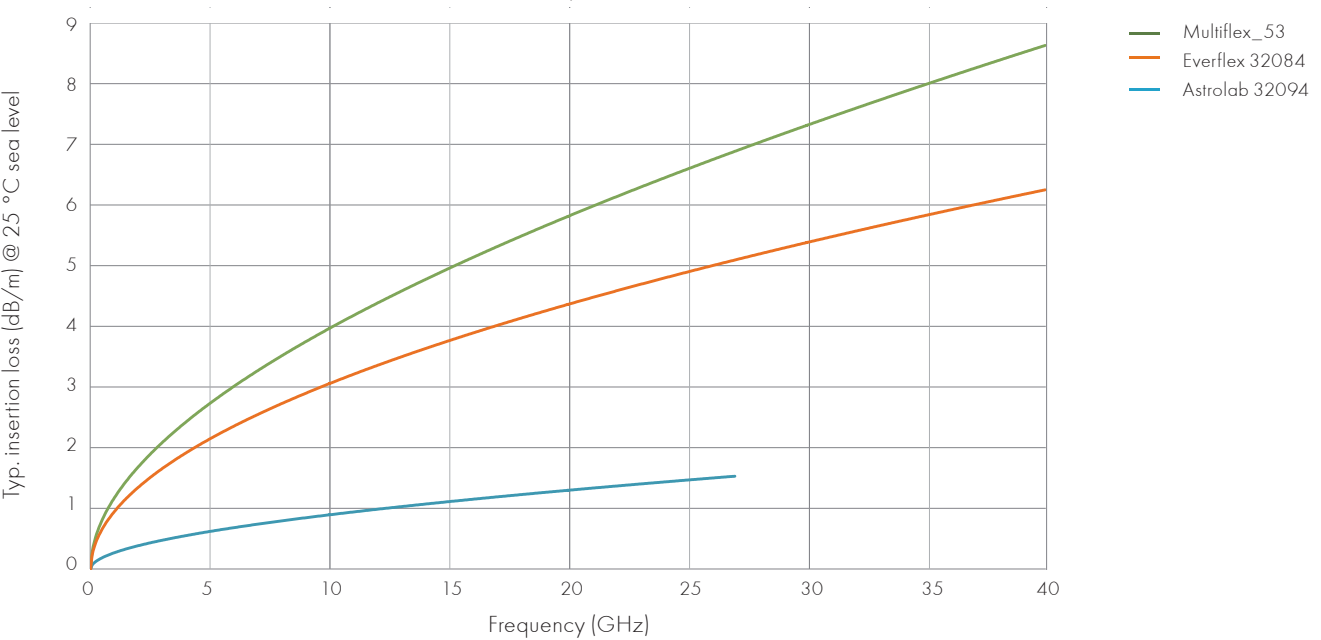
Attenuation (nominal values at +25 °C ambient temperature)
