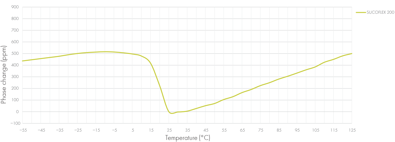
Phase stability versus temperature
