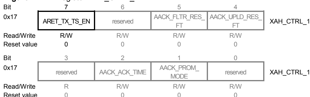
Figure 11-14. Register XAH_CTRL_1.
