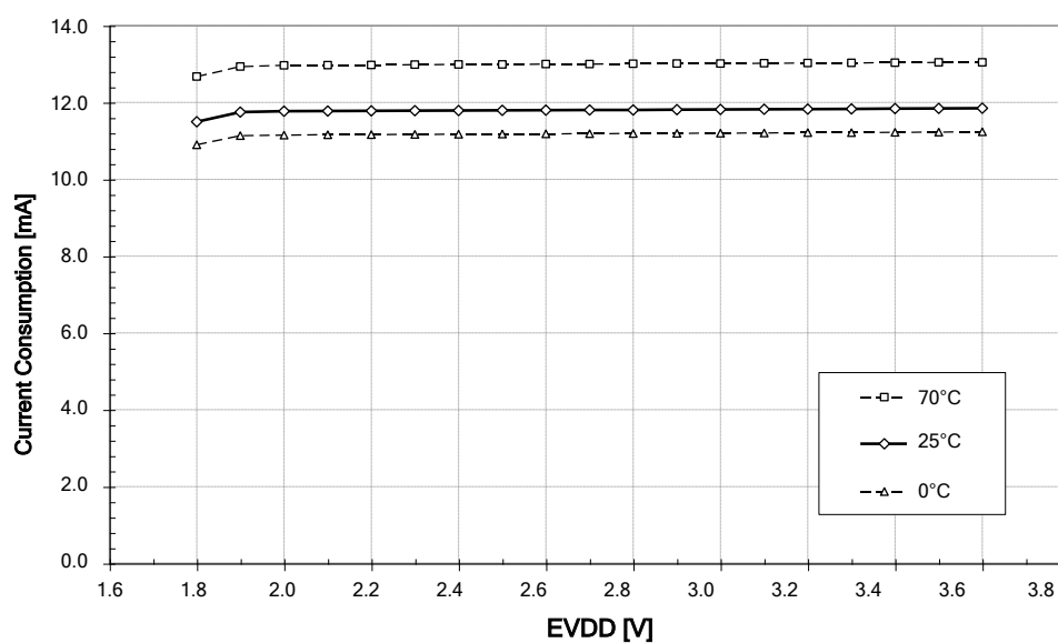
Figure 13-4. Current Consumption in RX_ON State – High Sensitivity.
