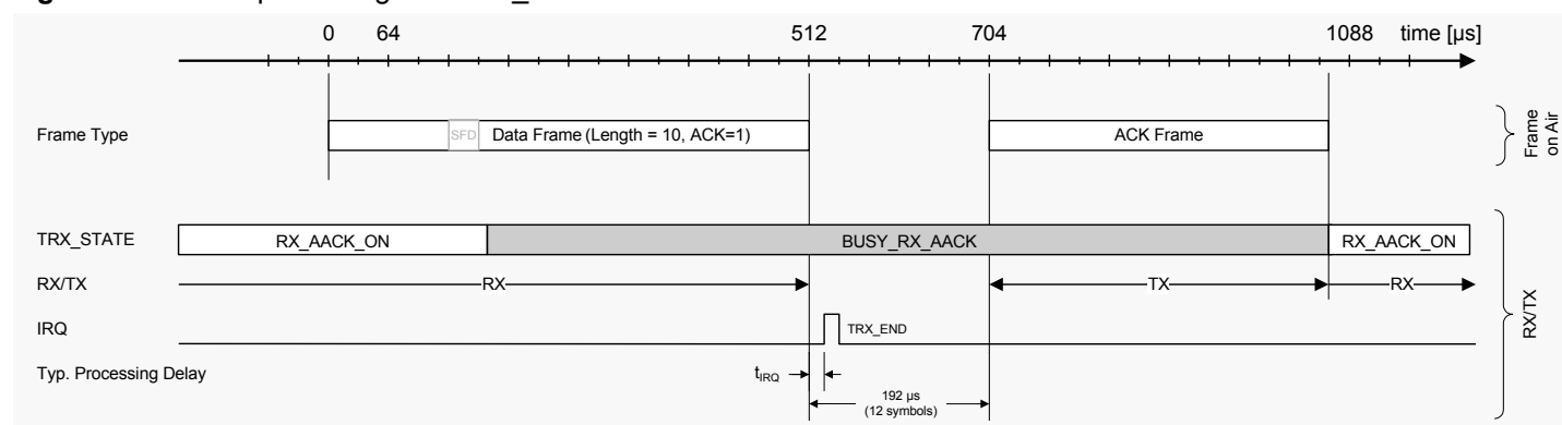
Figure 7-13. Example Timing of an RX_AACK Transaction.
