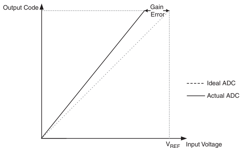
Figure 4-68. Gain Error
