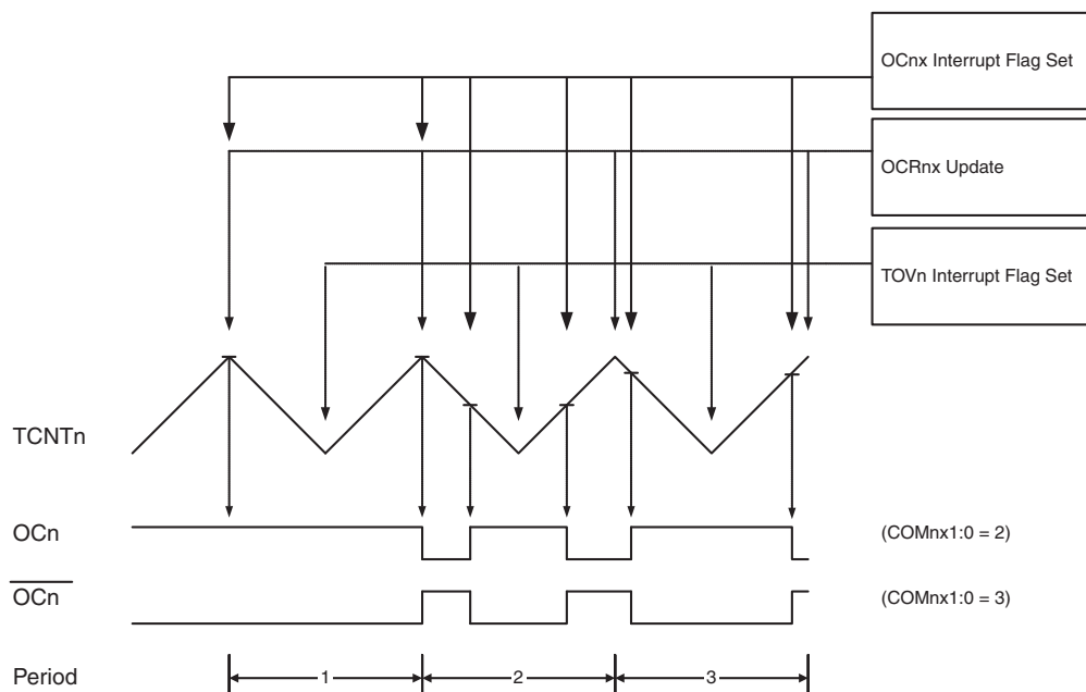
Figure 4-32. Phase Correct PWM Mode, Timing Diagram
