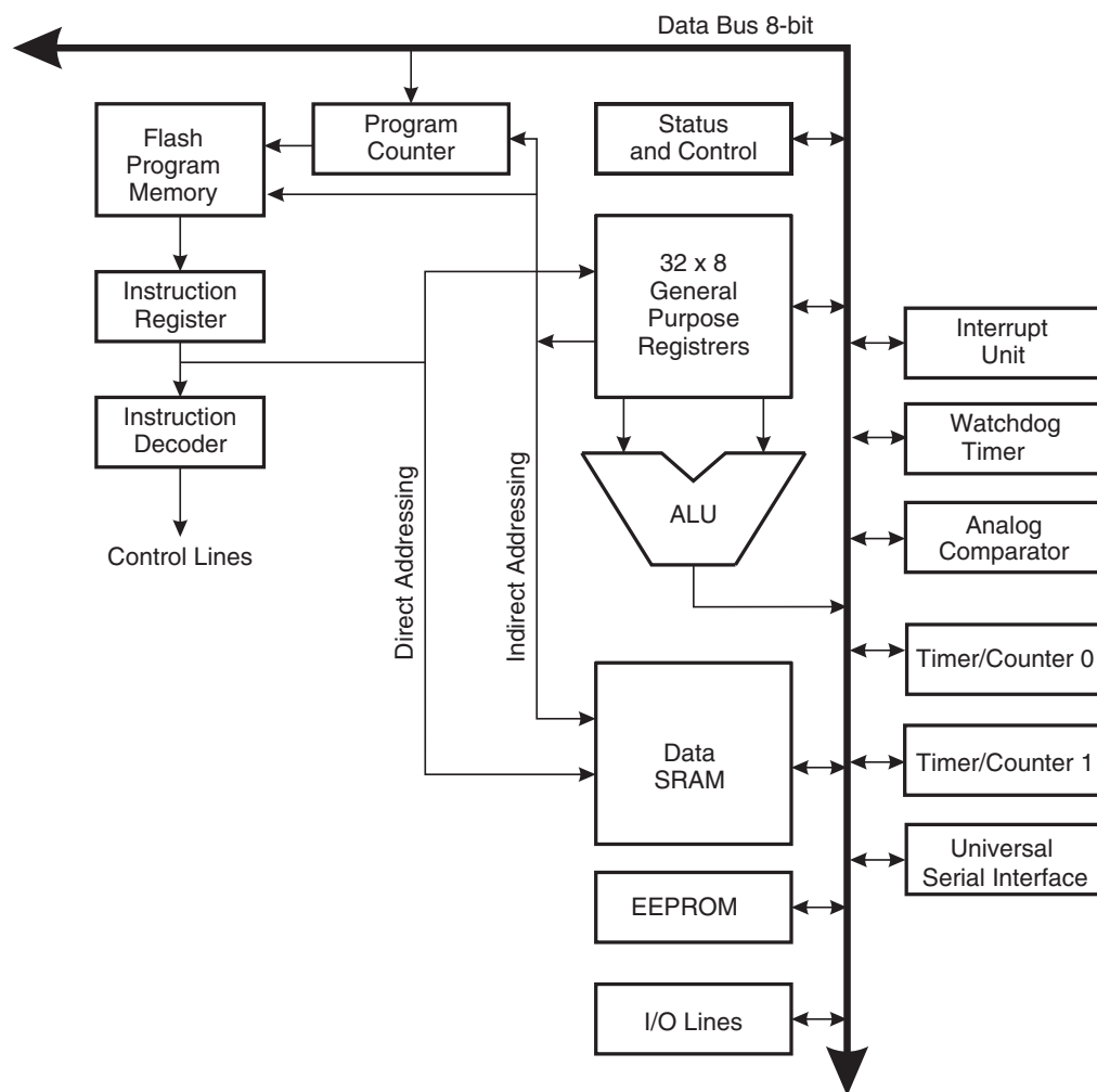
Figure 4-2. Block Diagram of the Atmel AVR Architecture
