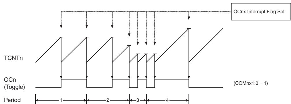
Figure 4-30. CTC Mode, Timing Diagram
