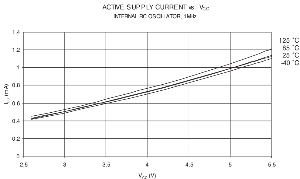
Figure 8-9. Active Supply Current vs. V_{CC} (Internal RC Oscillator, 1MHz)
