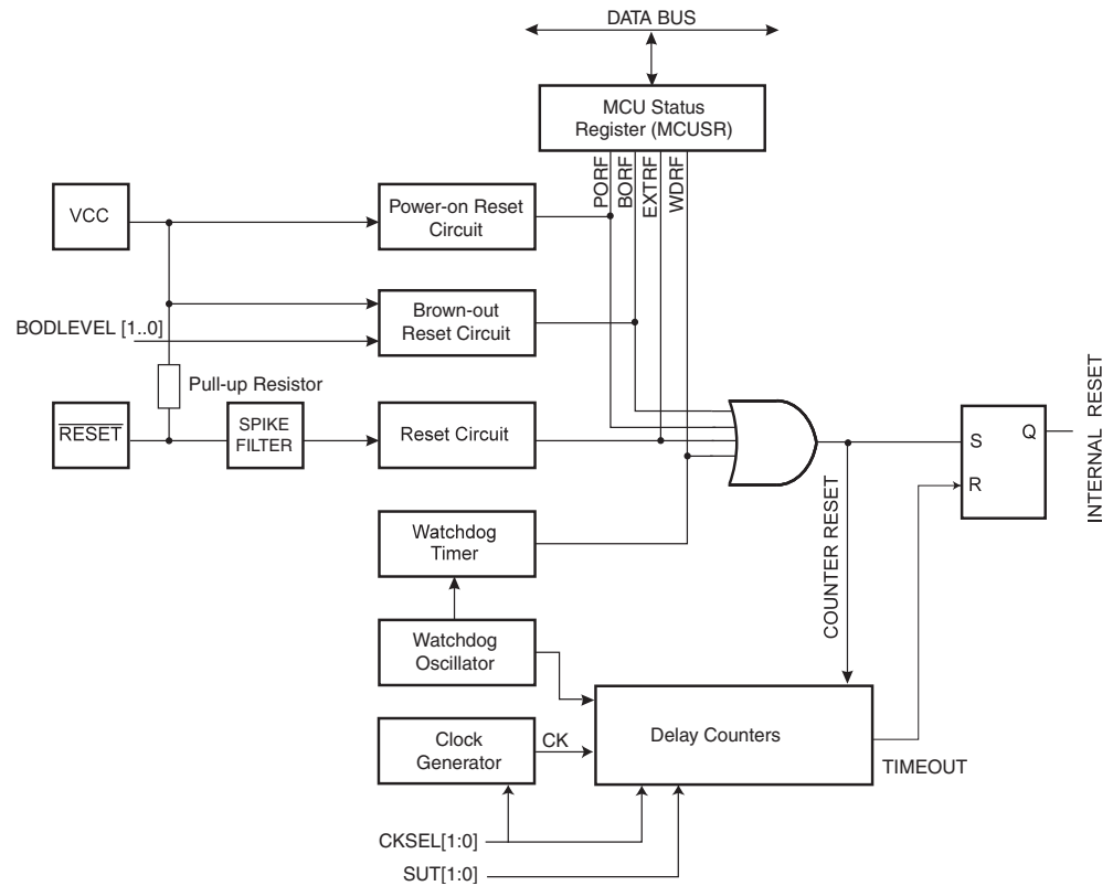
Figure 4-13. Reset Logic
