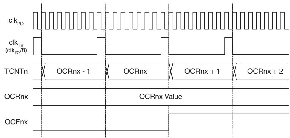
Figure 4-47. Timer/Counter Timing Diagram, Setting of OCF1x, with Prescaler ( f_{\text{clk}_{I/O}}/8 )
