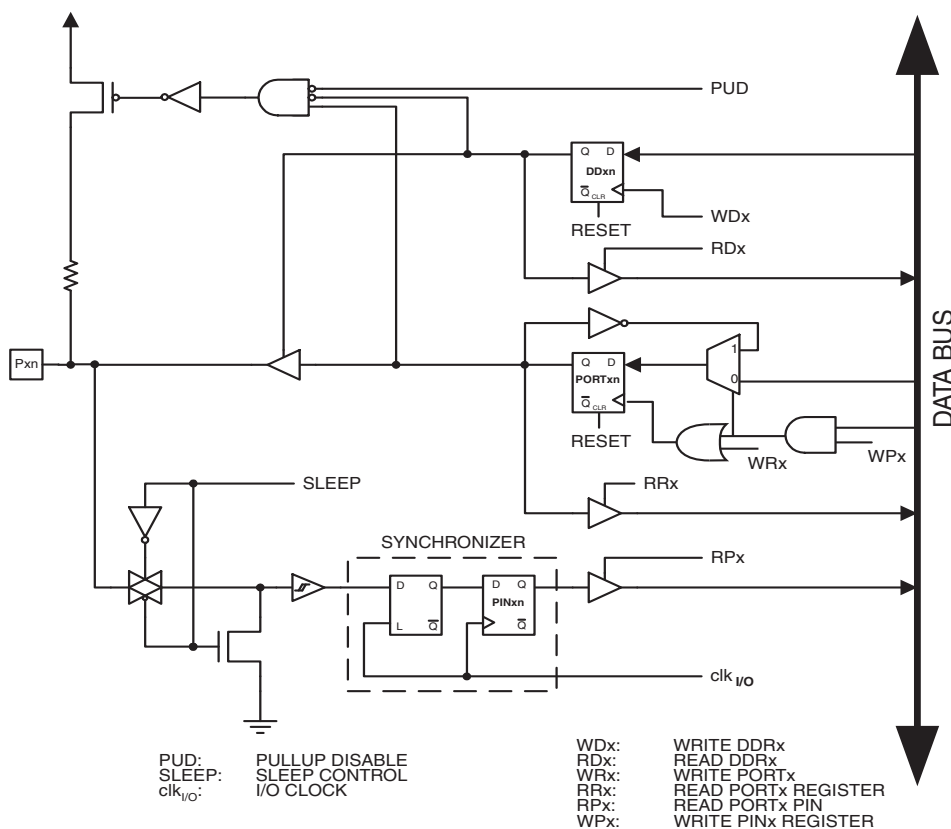
Figure 4-22. General Digital I/O (1)
