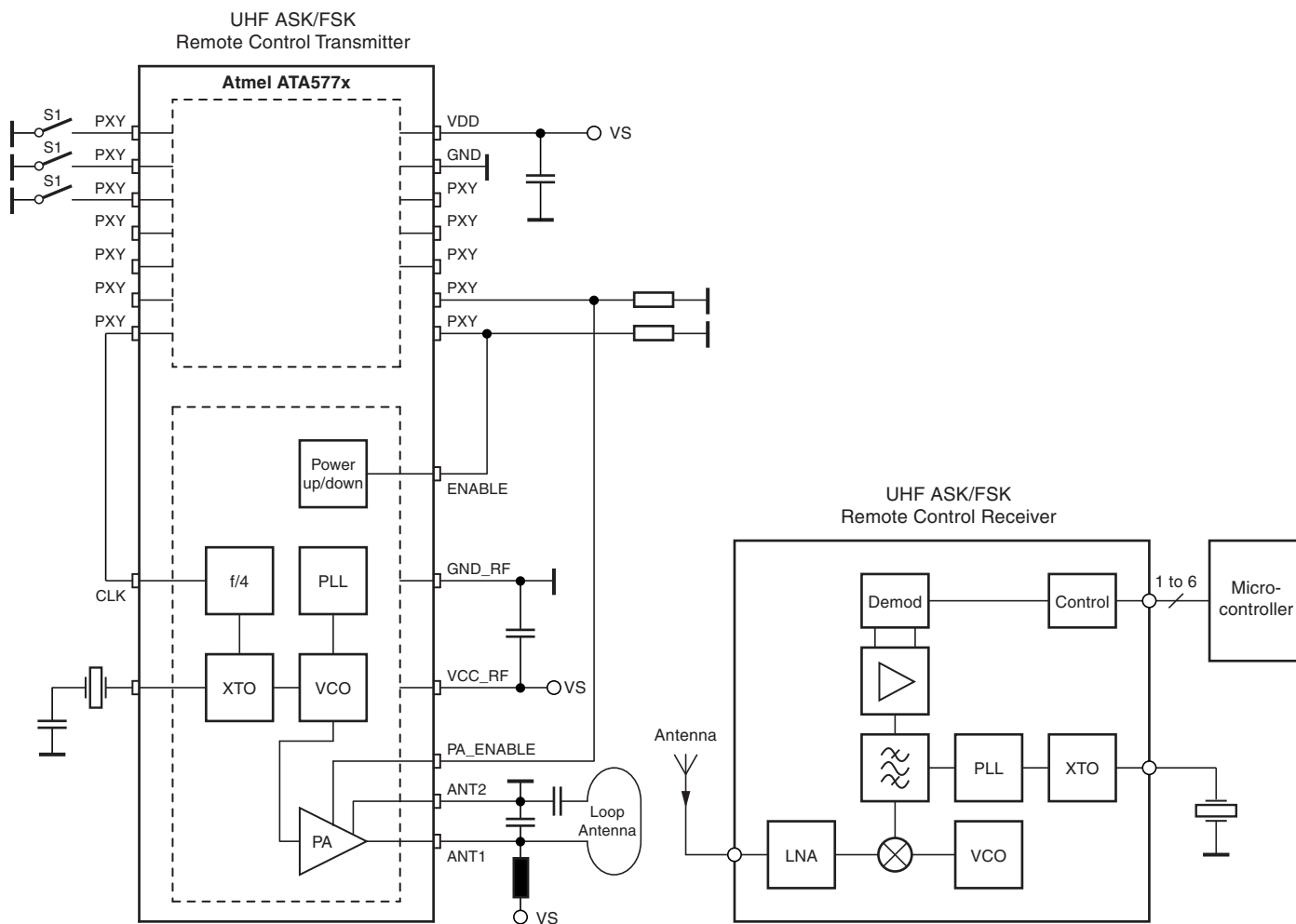
Figure 1-1. ASK System Block Diagram
