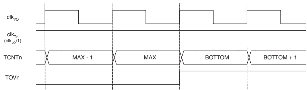
Figure 4-33. Timer/Counter Timing Diagram, no Prescaling
