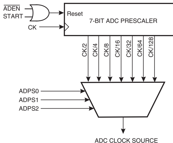
Figure 4-61. ADC Prescaler
