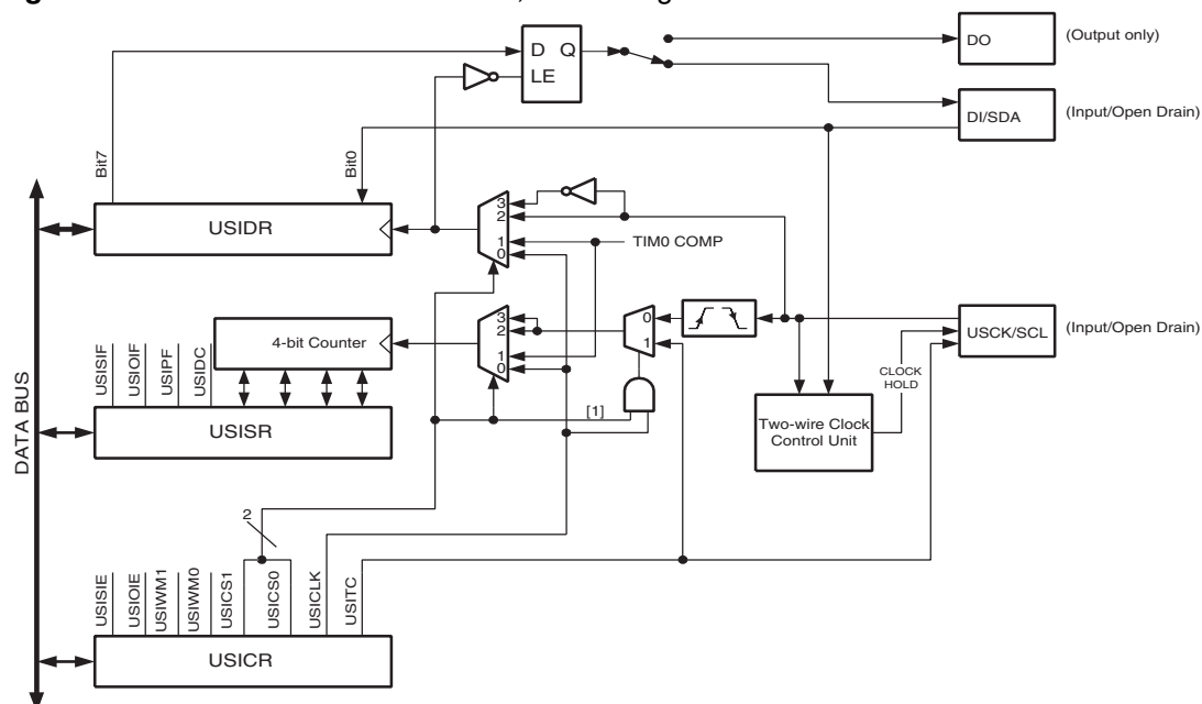
Figure 4-52. Universal Serial Interface, Block Diagram
