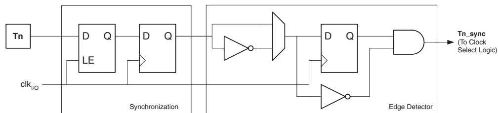
Figure 4-50. T0 Pin Sampling
