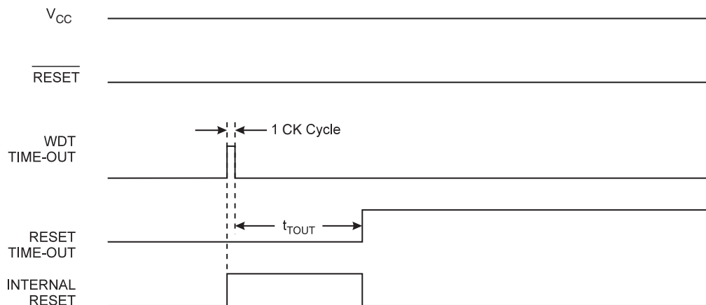
Figure 4-18. Watchdog Reset During Operation
