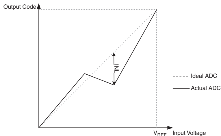
Figure 4-69. Integral Non-linearity (INL)
