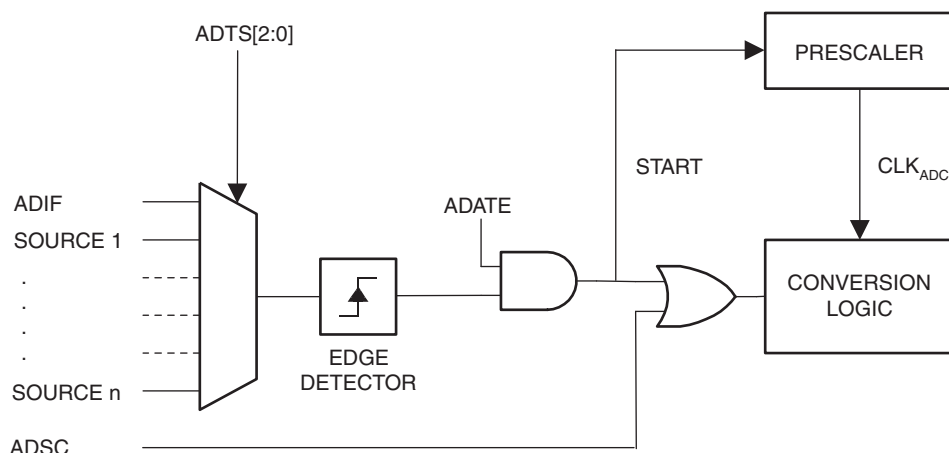
Figure 4-60. ADC Auto Trigger Logic
