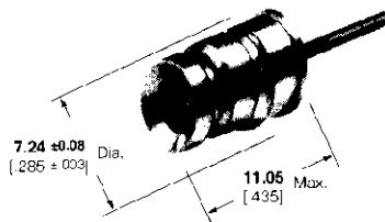
RG-405 Semi-Rigid Cable - Part No. 413012-1 1.19 [047] Semi-Rigid Cable - Part No. 413025-1
