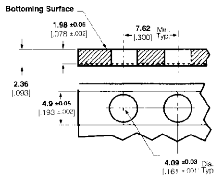
Recommended Panel Layout
