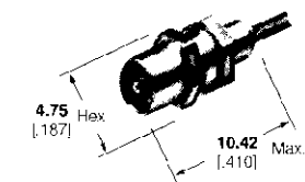
1.19 [047] Semi-Rigid Cable - Part No. 413024-1
